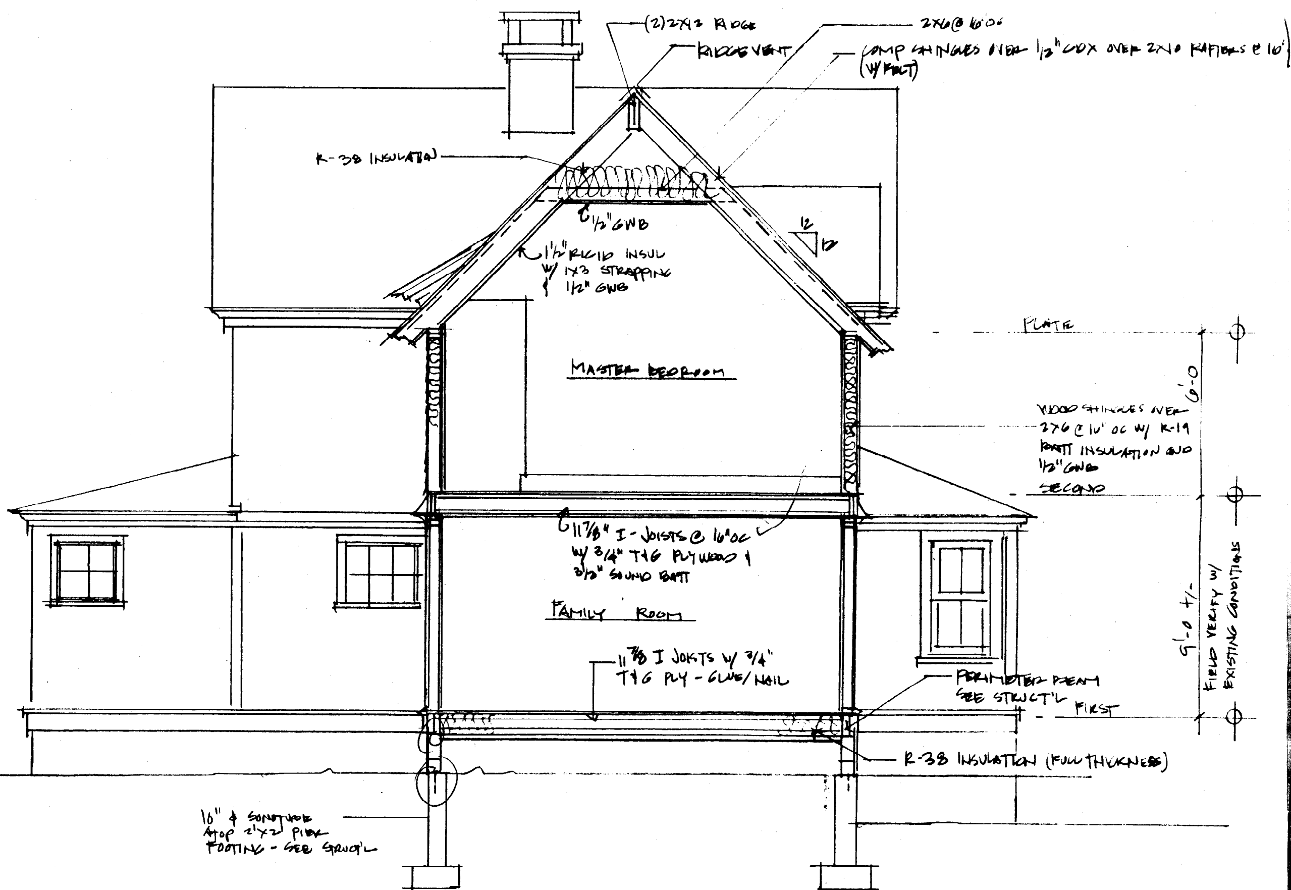
BUILDING SECTION
