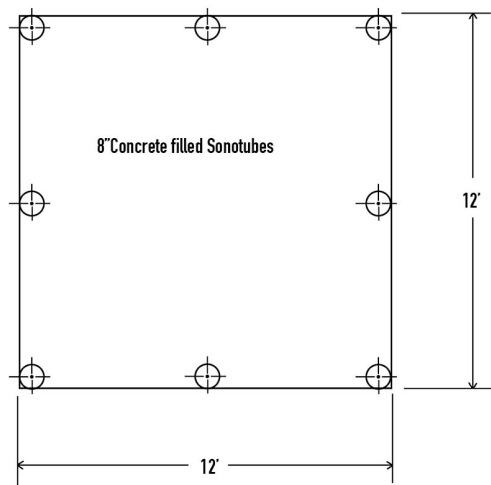
FOUNDATION PLAN
