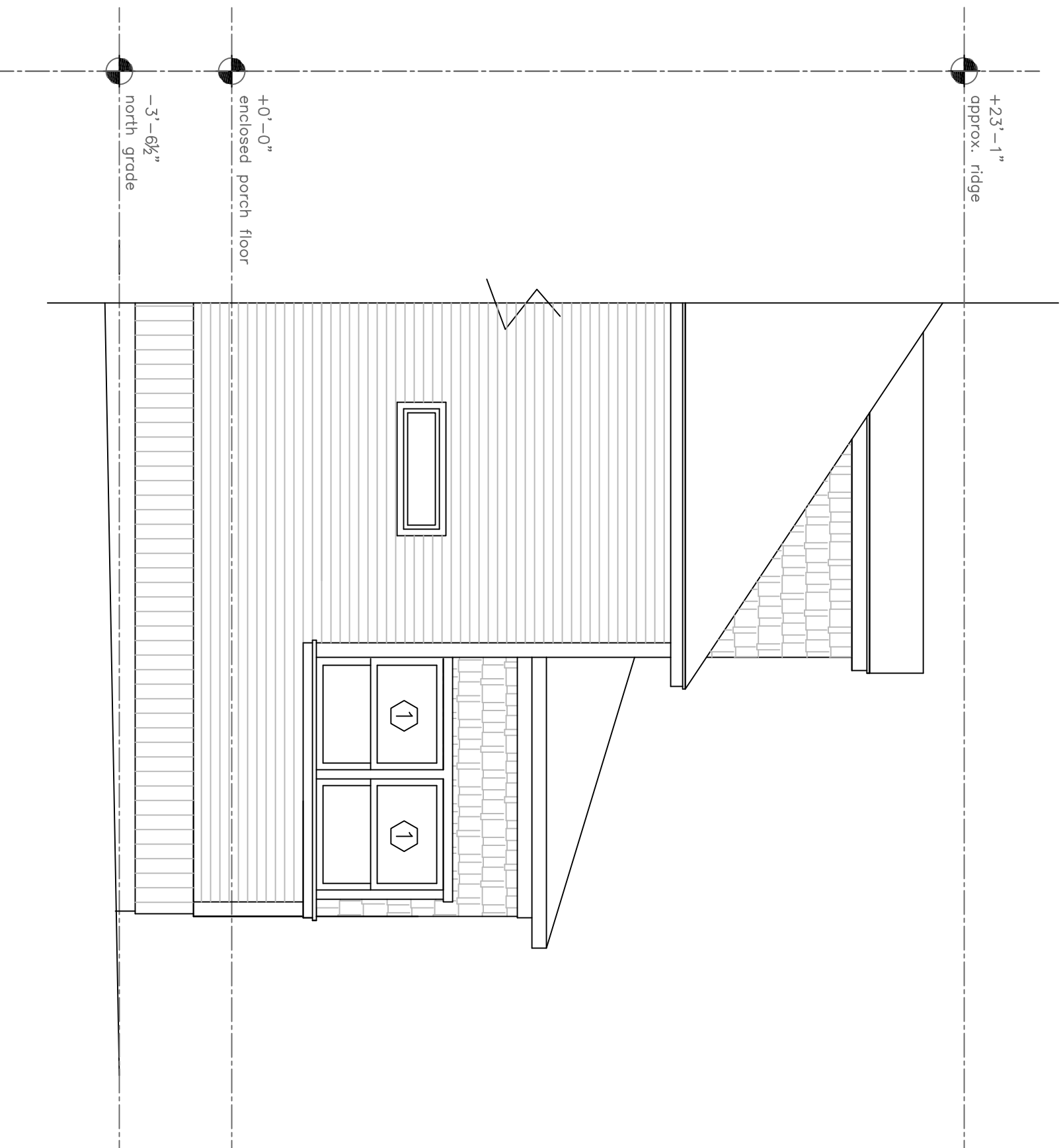
A Proposed East Elevation \frac{1}{4}'' = 1' - 0''
