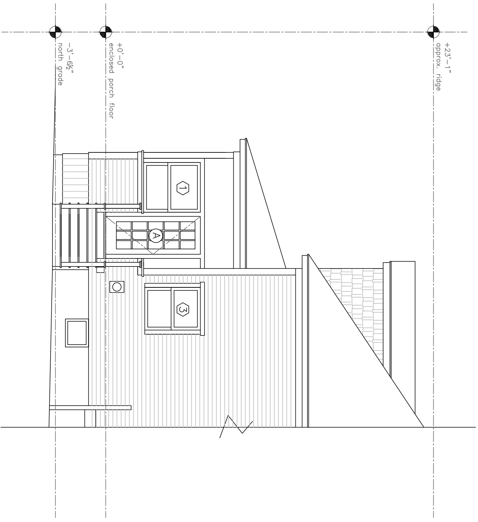
A Proposed West Elevation \frac{1}{4}'' = 1' - 0''
