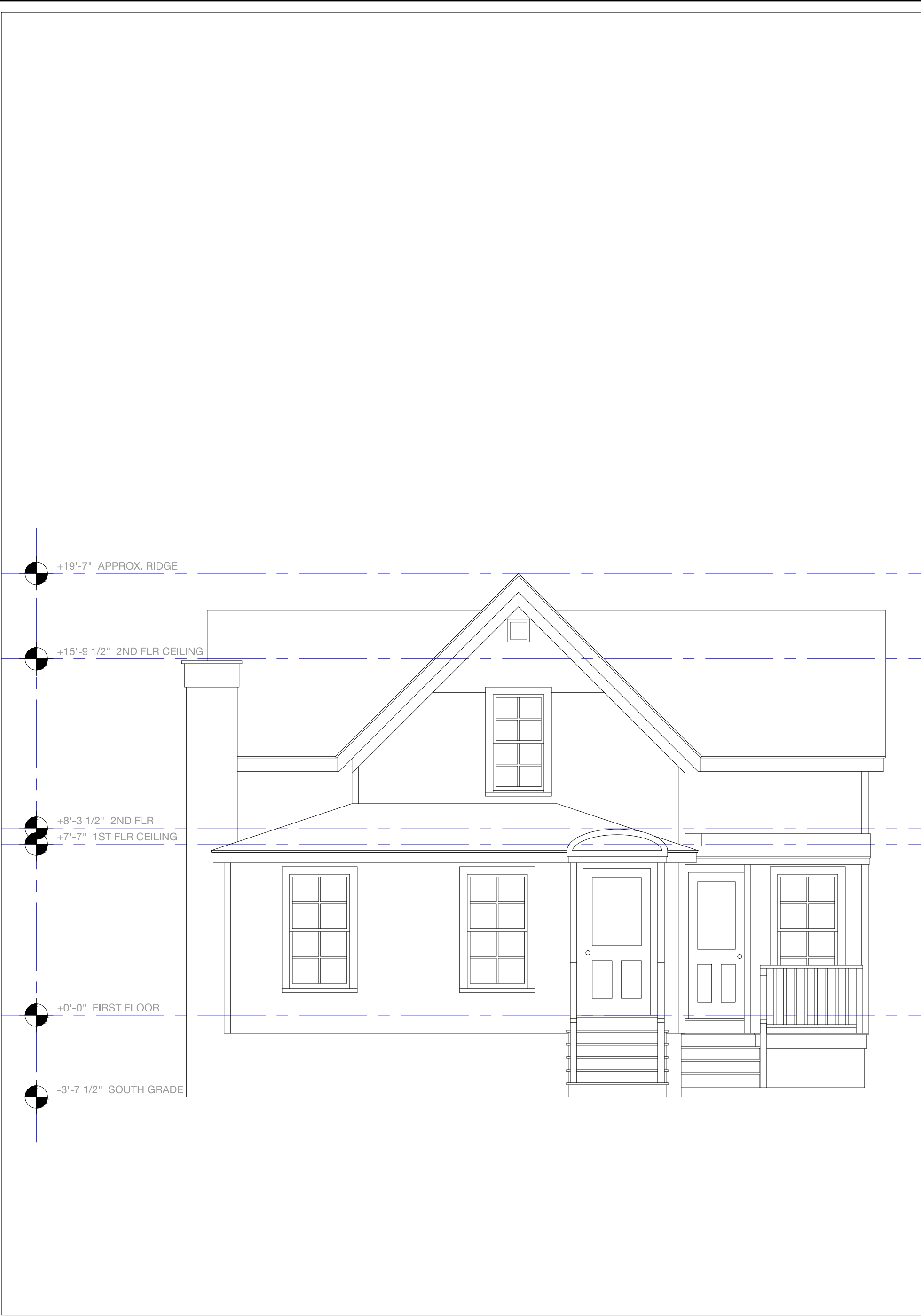
A Existing South Elevation
