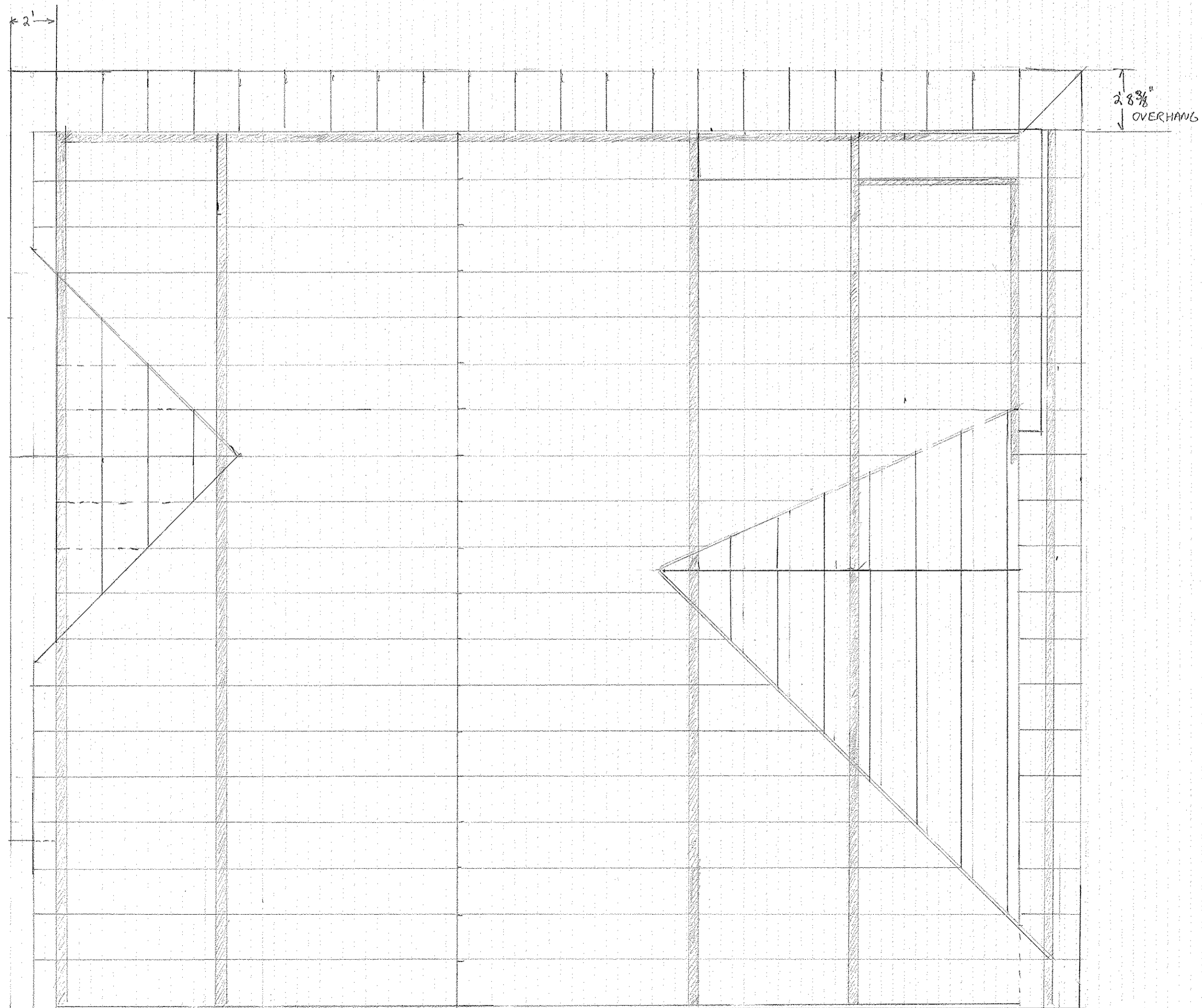
ROOF FRAMING PLAN 1/4" = 1'
