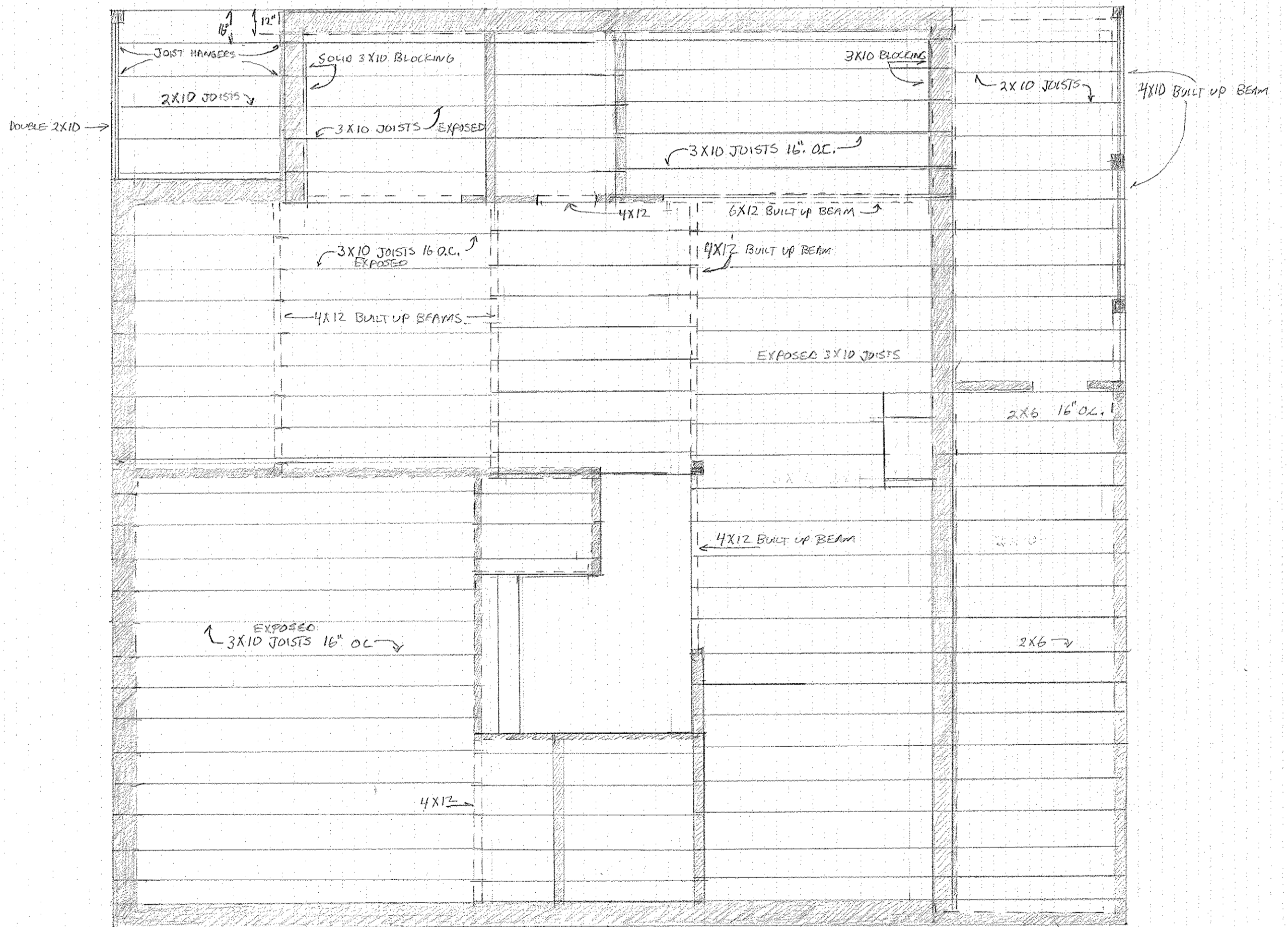
SECOND FLOOR FRAMING PLAN SCALE 1/4" = 1' K-1
