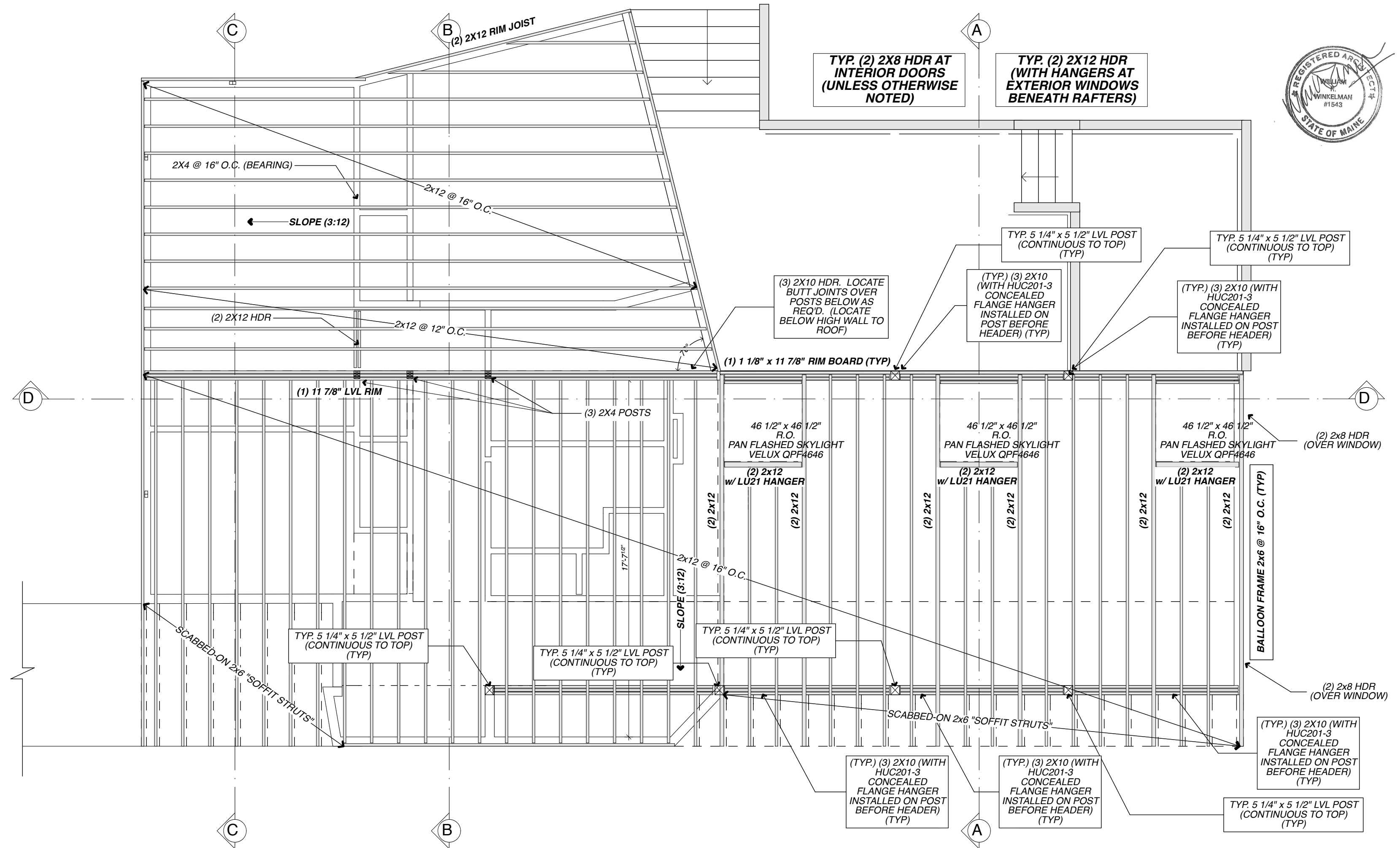
ROOF FRAMING PLAN: 1/4" = 1'-0"
