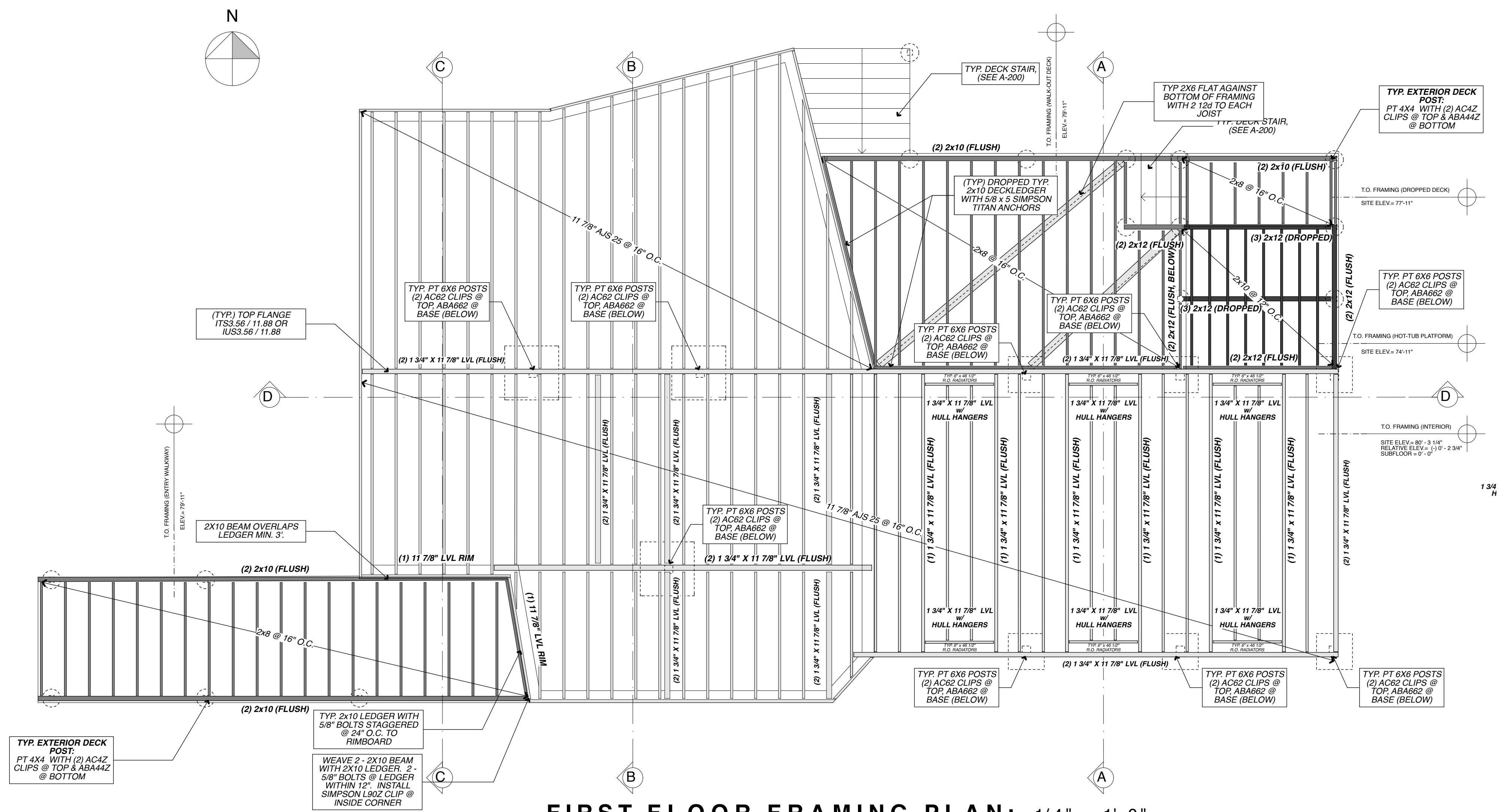
FIRST FLOOR FRAMING PLAN: 1/4" = 1'-0"
