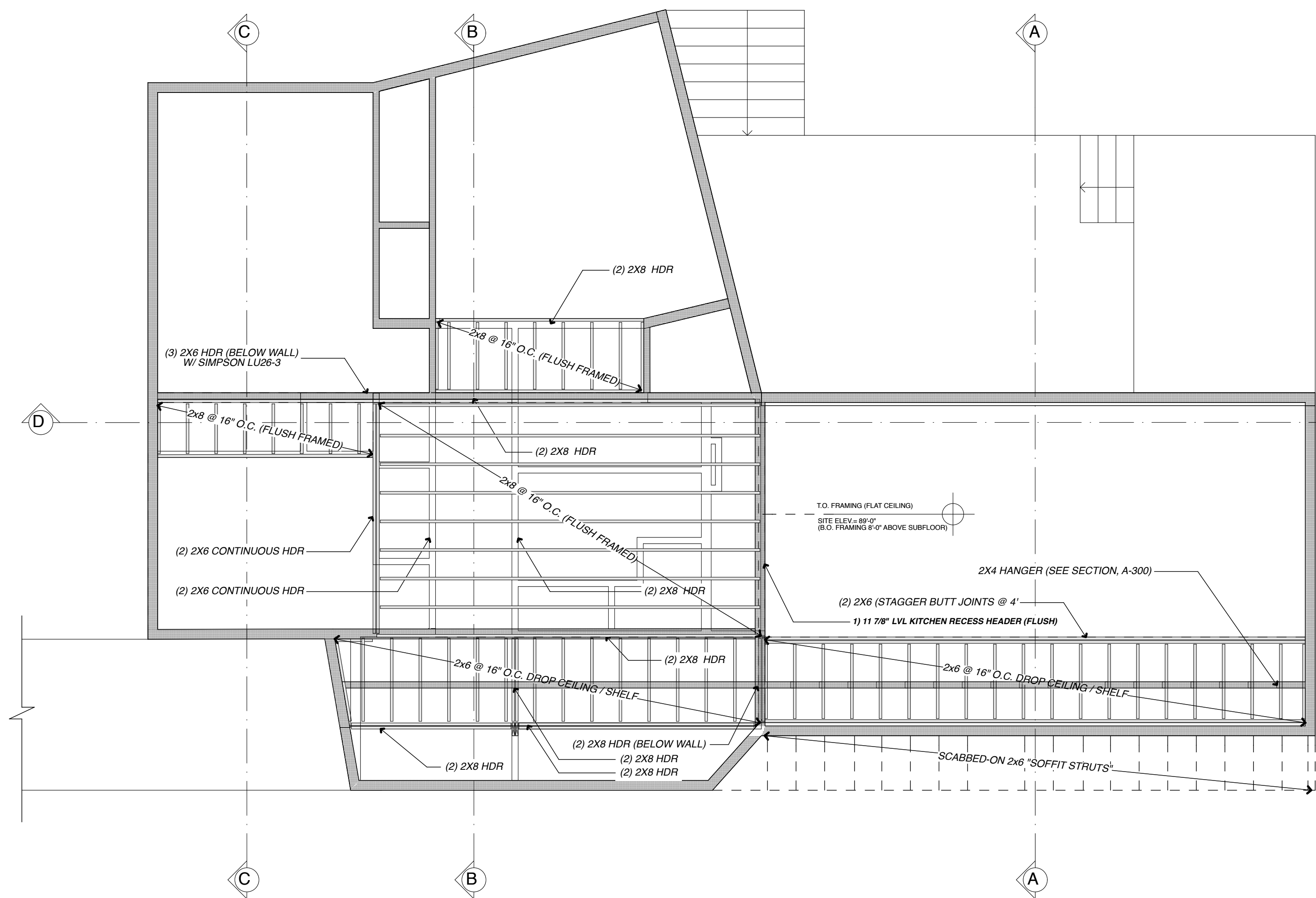
FLAT CEILING FRAMING PLAN: 1/4" = 1'-0"
