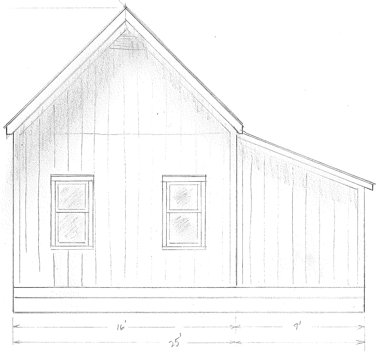
SOUTH ELEVATION
