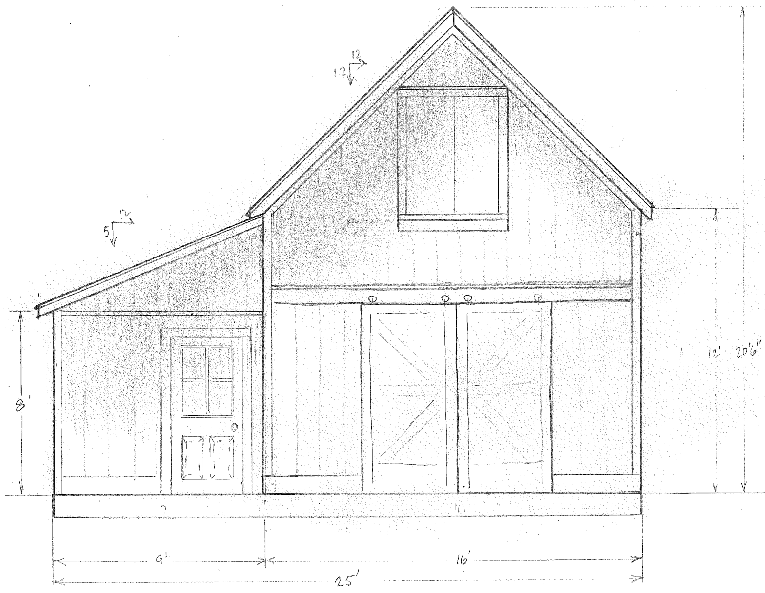
NORTH ELEVATION
