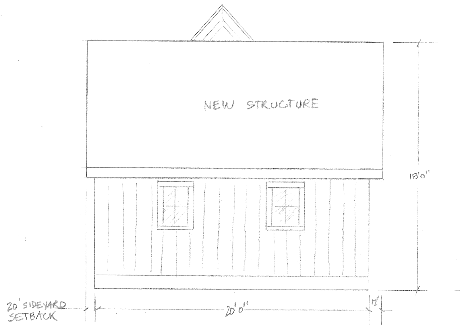
WEST ELEVATION
