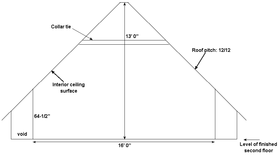
Second floor section w/ceiling height (all existing; no partitions, windows, or doors are being altered)
