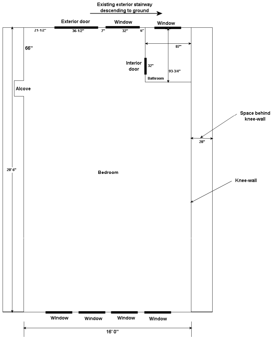
Second floor plan (all existing; no partitions, windows, or doors are being altered)
