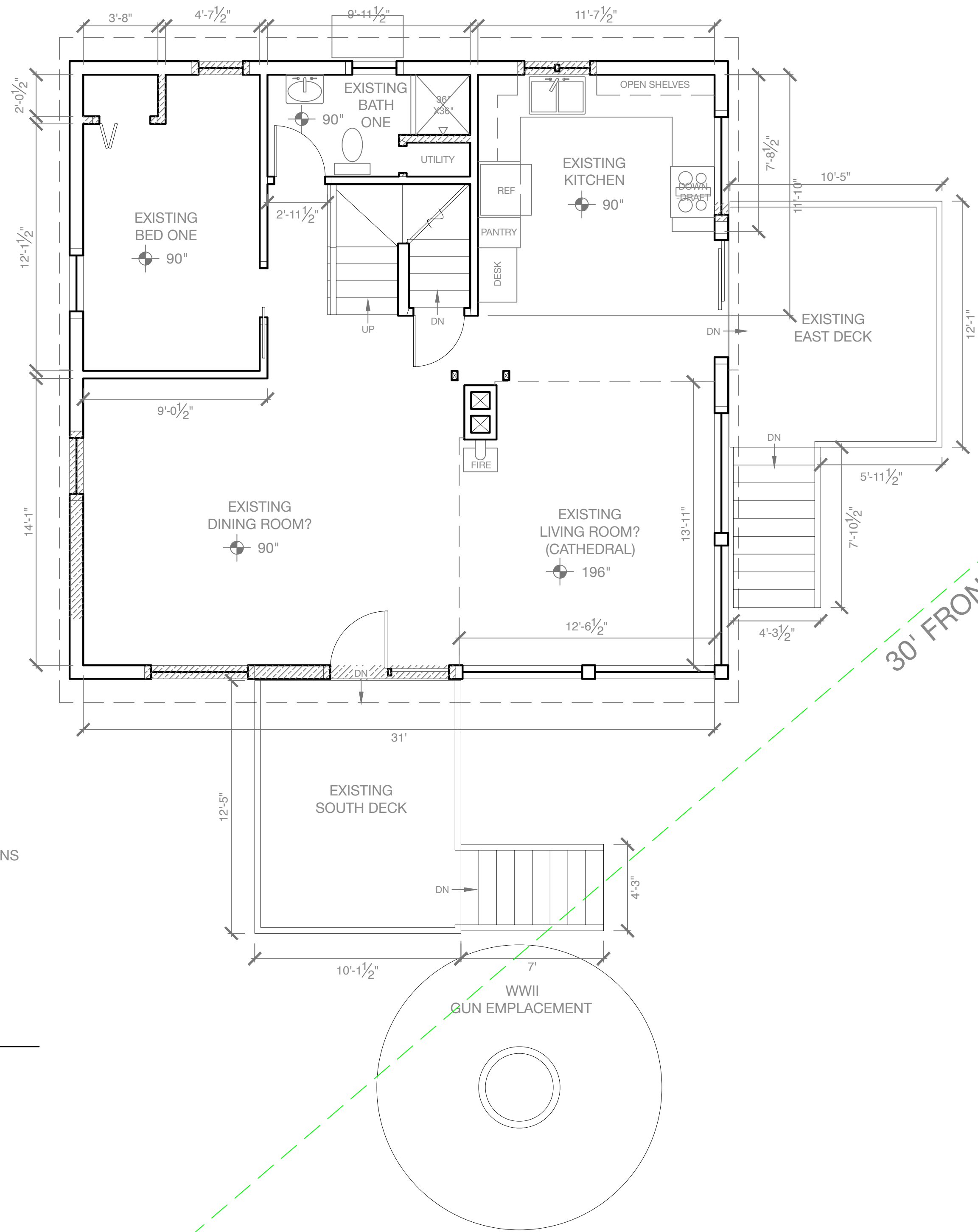
A Existing First Floor Plan
