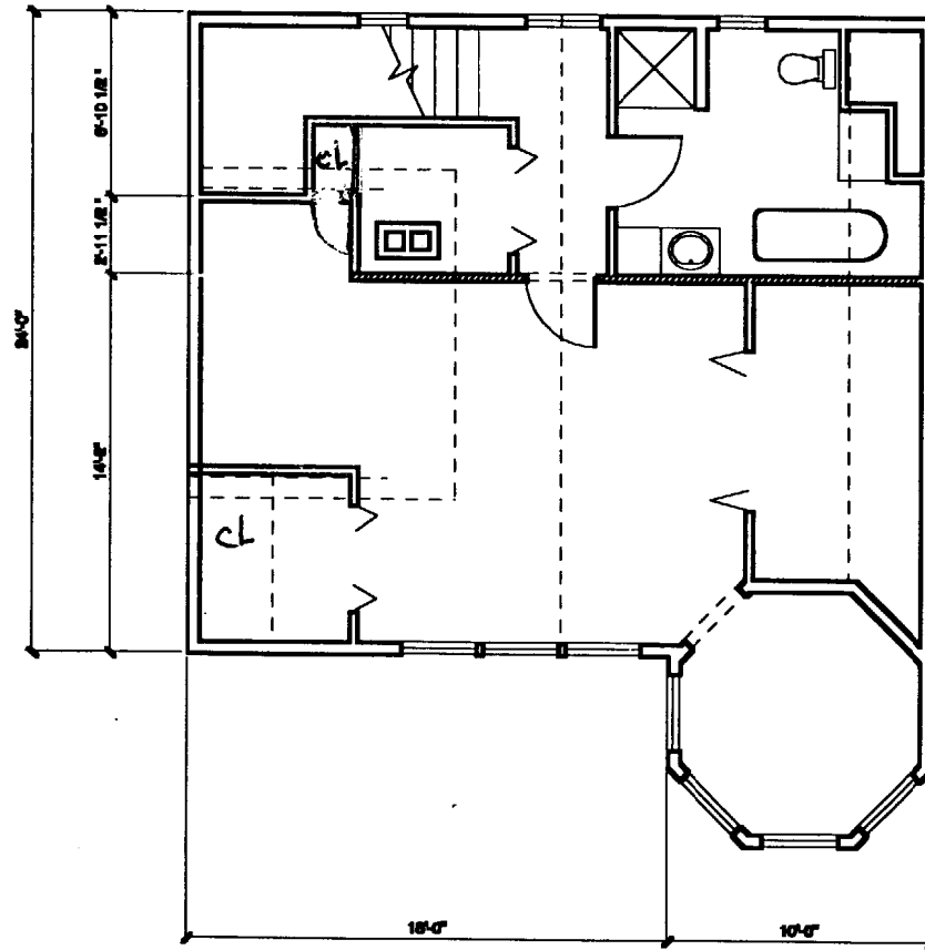
10 second floor plan 1/8"=1'-0"
