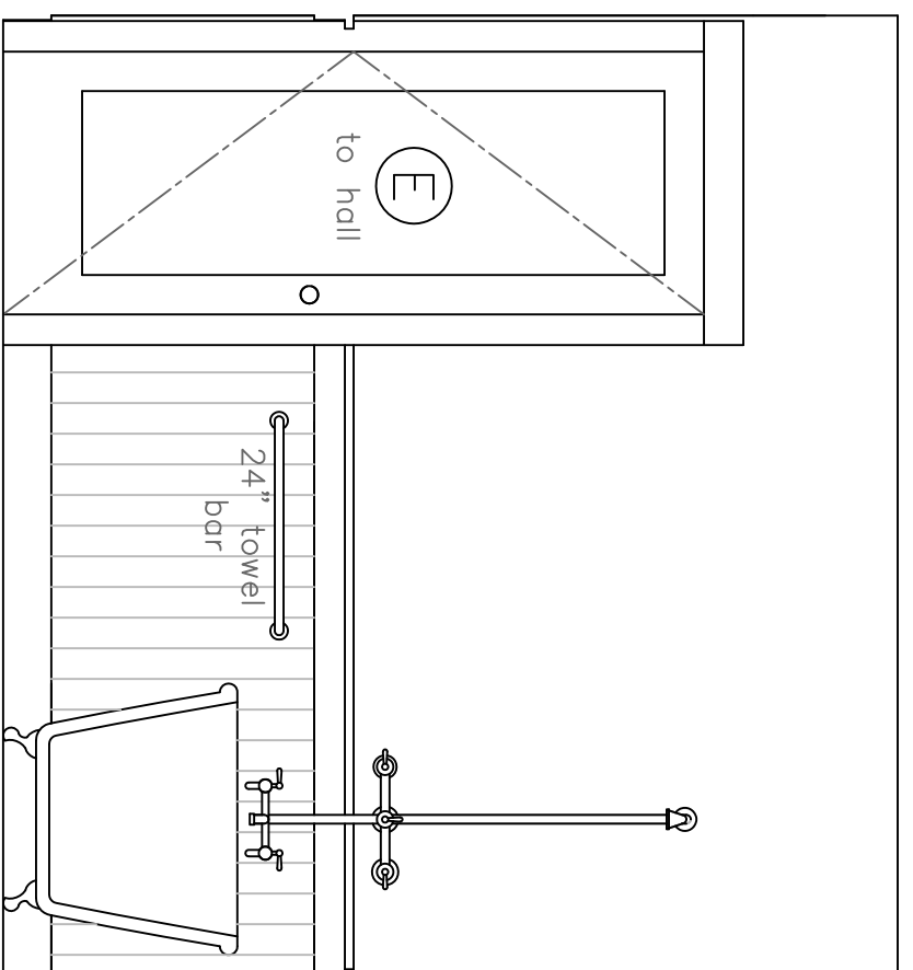
C Proposed Second Floor Bath: South \frac{1}{2}'' = 1'-0''
