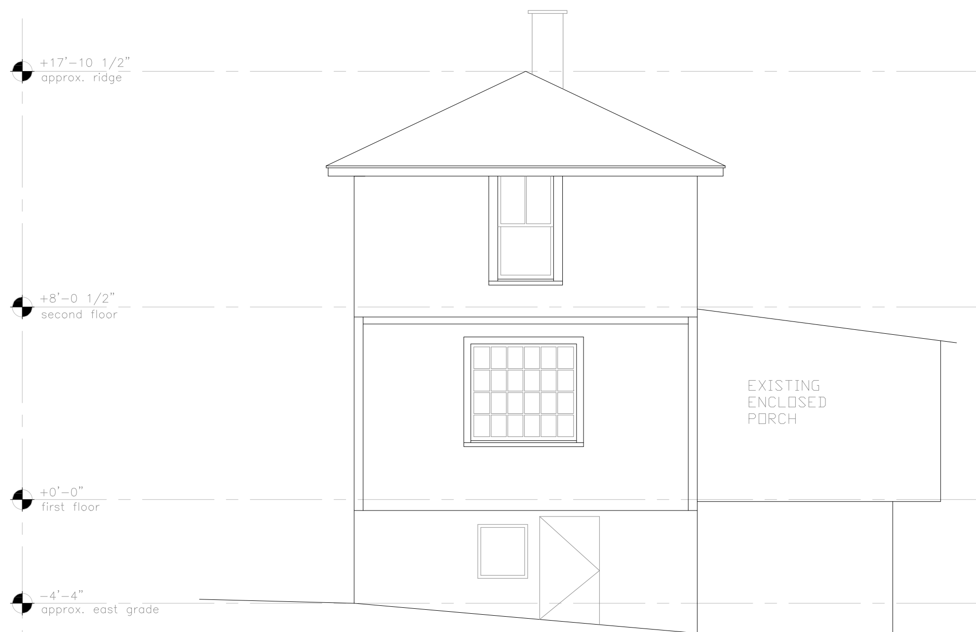
(A) Existing North Elevation 1/4" = 1'-0"
