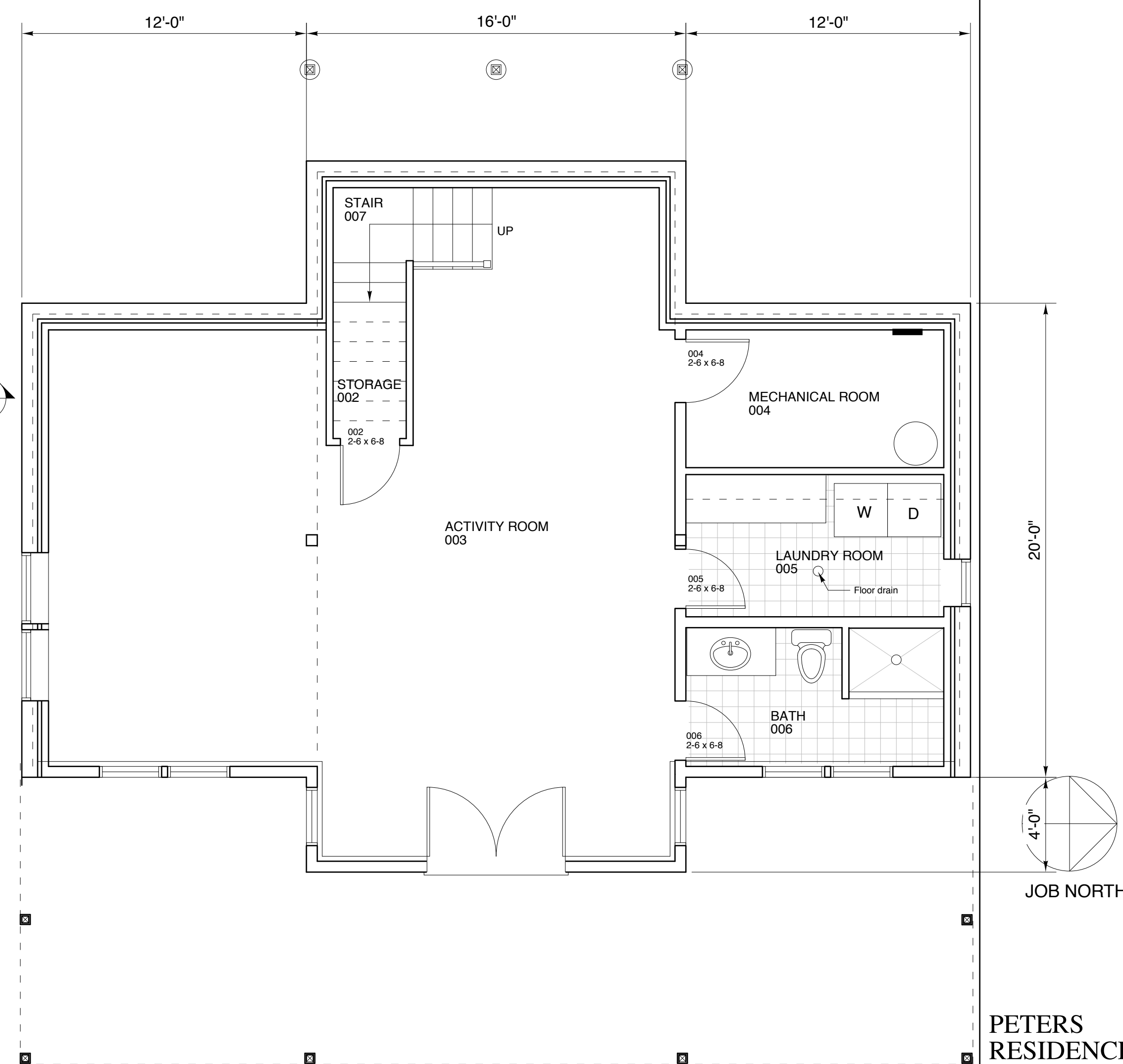
BASEMENT
