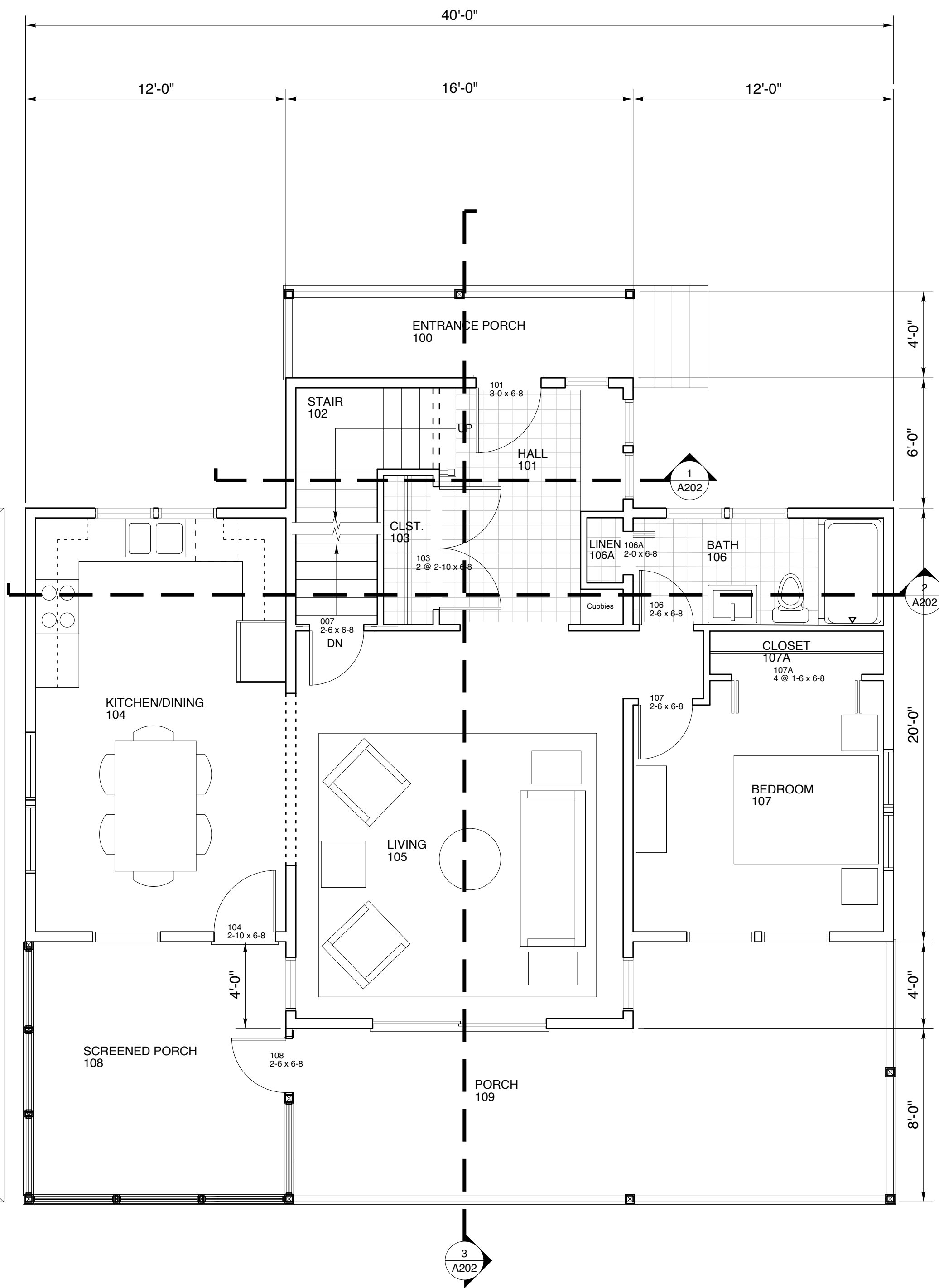
FIRST FLOOR
