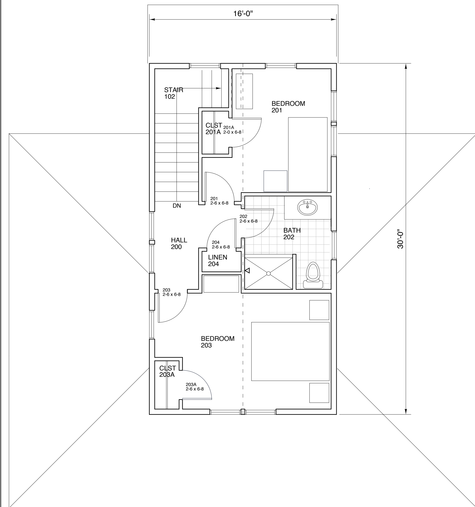
SECOND FLOOR
