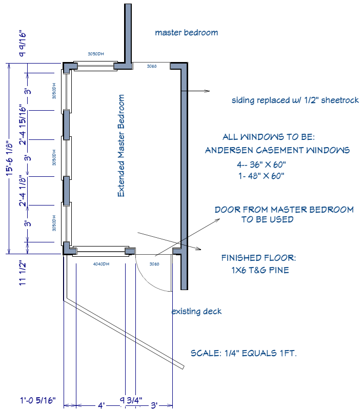
page--A-7 proposed floor plan for bedroom extension
