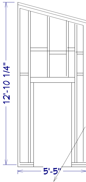
2 X 6 STUD WALL W/ R-32 FIBERGLASS INSULATION
