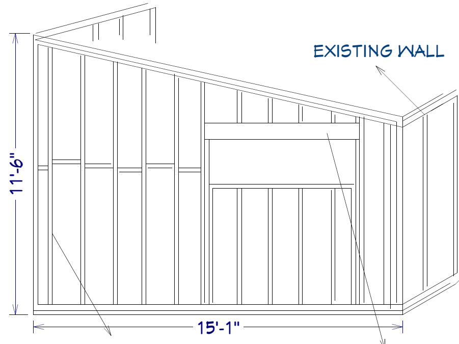
2 X 6 STUD WALL W/ - R-32 FIBERGLASS INSULATION
