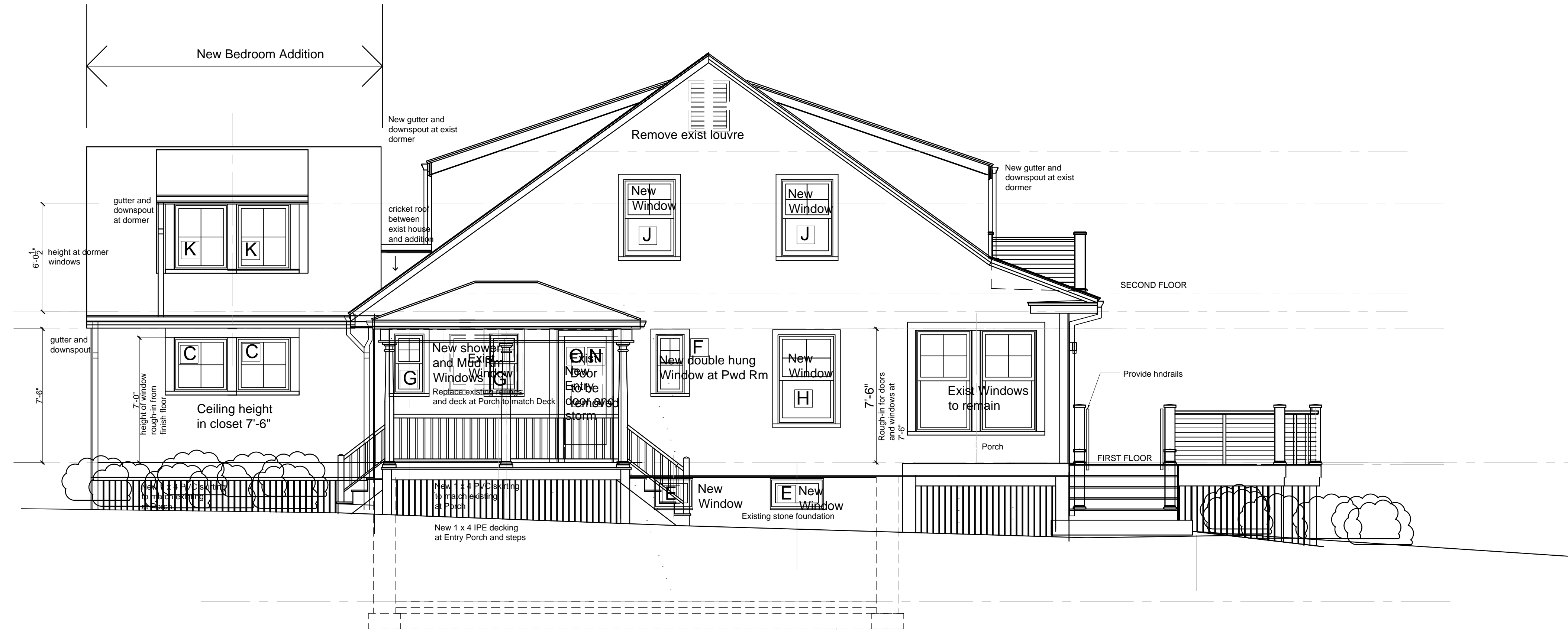
2 Elevation - North
