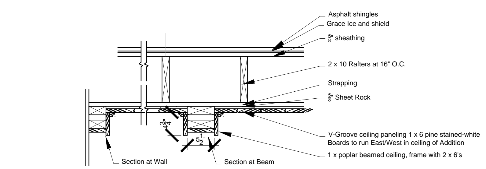
Section-D Ceiling Beam Details-Sections At new Addition Bedroom and Loft scale: 1" = 1'-0"
