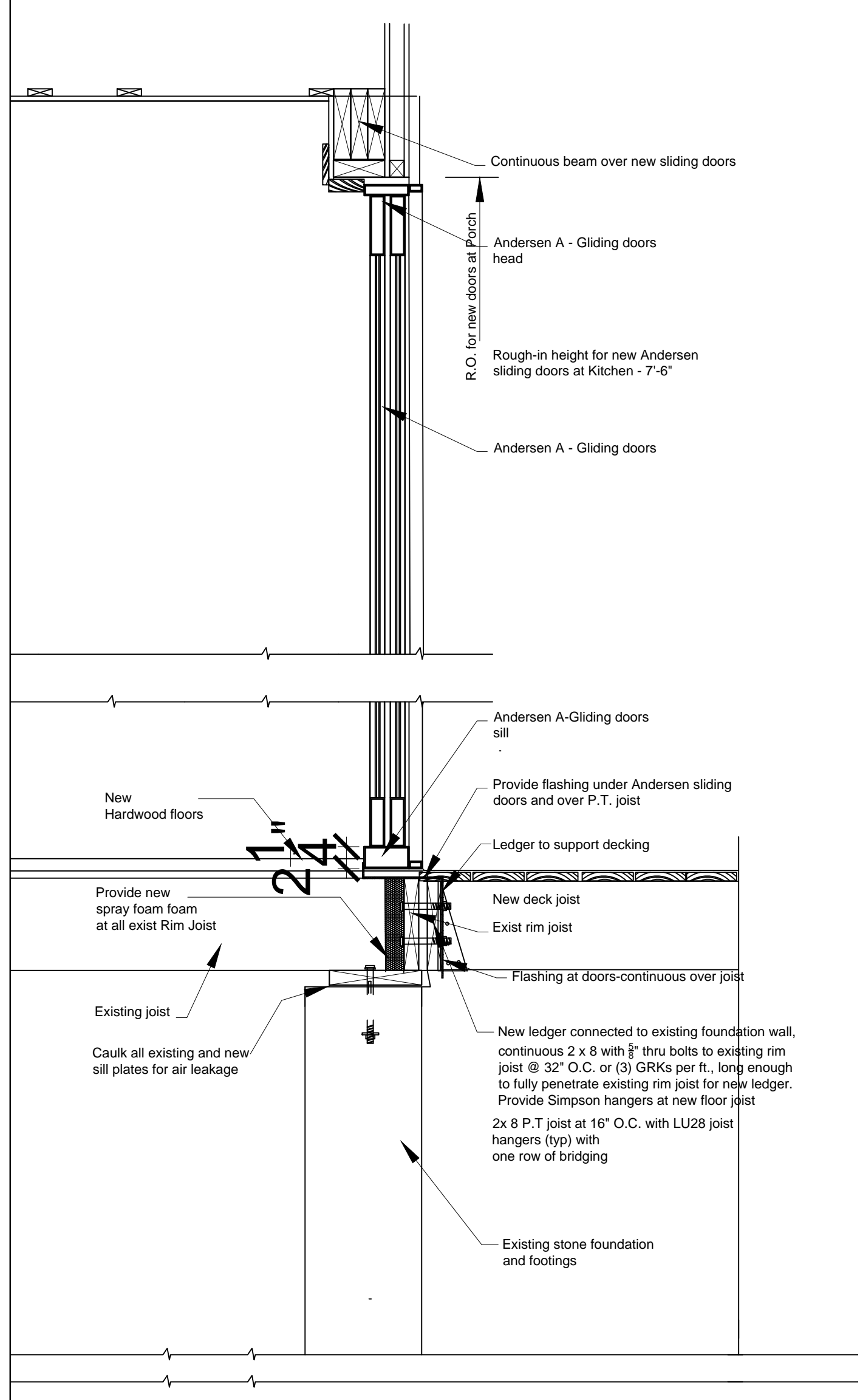
Section-A First Floor Deck-off Kitchen/Dining Area scale: 1" = 1'-0"
