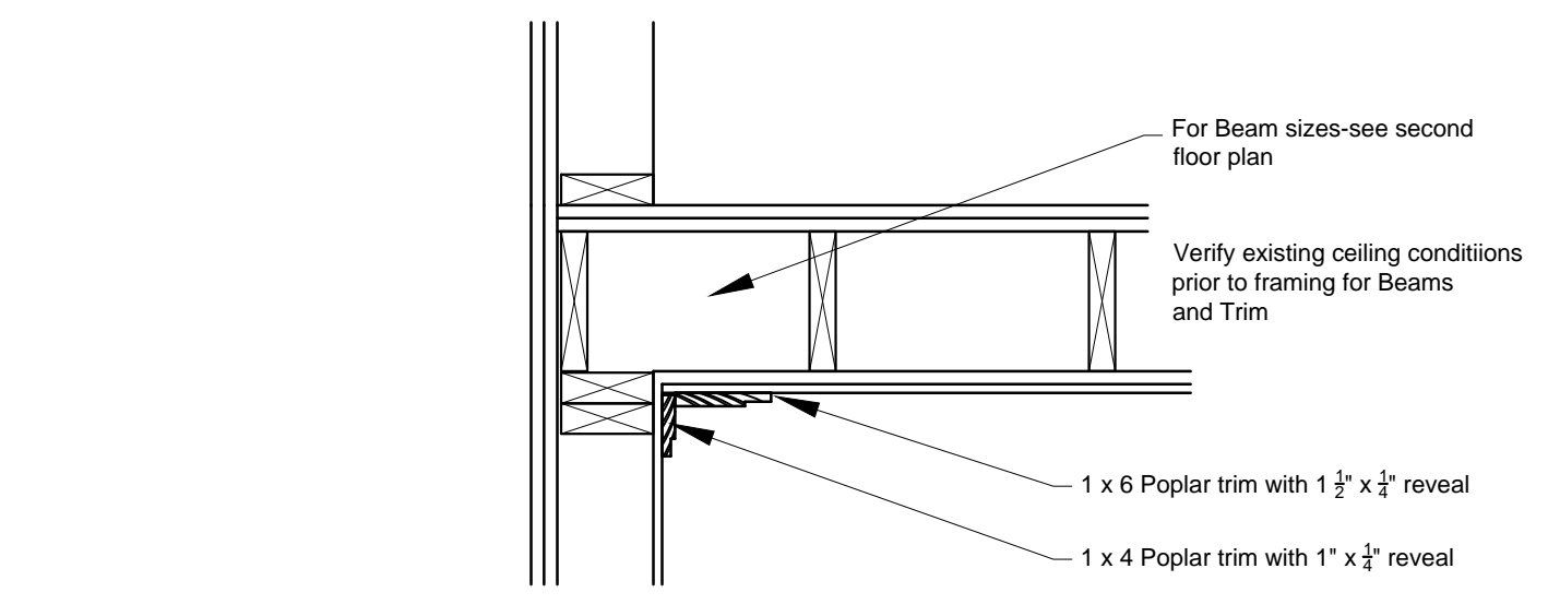
Section-F Typical Ceiling Wall Crown Section At Living Room, Kitchen and Hall scale: 1" = 1'-0"
