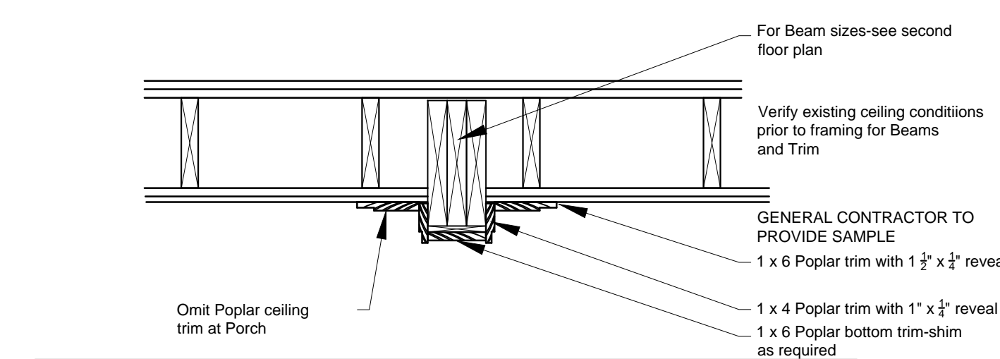
Section-E Typical Ceiling Beam Sections At Living Room and Hall scale: 1" = 1'-0"
