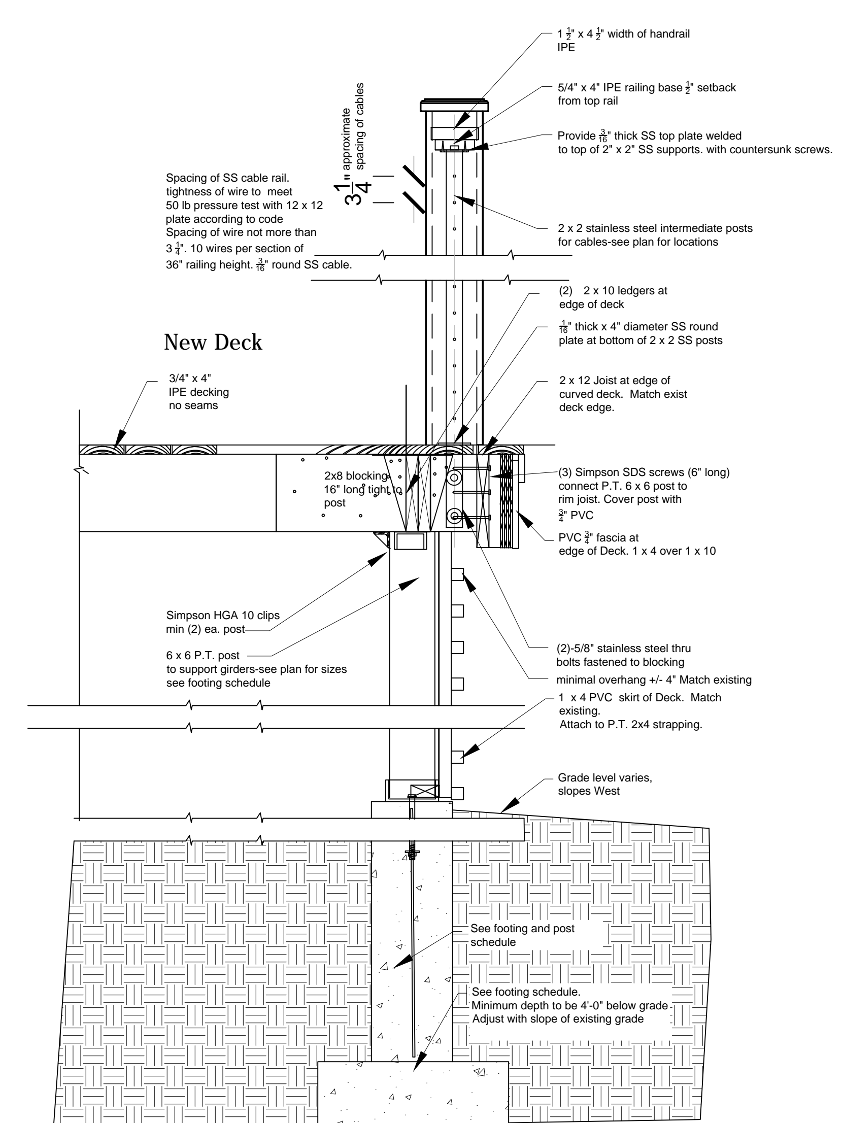
Section-B @ 2 x 2 SS post scale: 1" = 1'-0"
