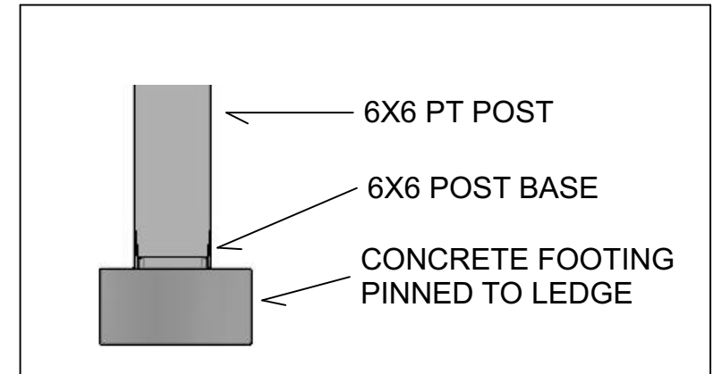
POST / FOOTING DETAIL 1/2" SCALE
