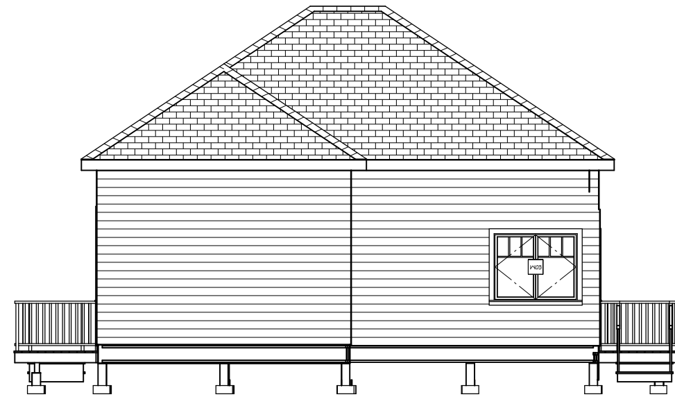
NORTH ELEVATION
