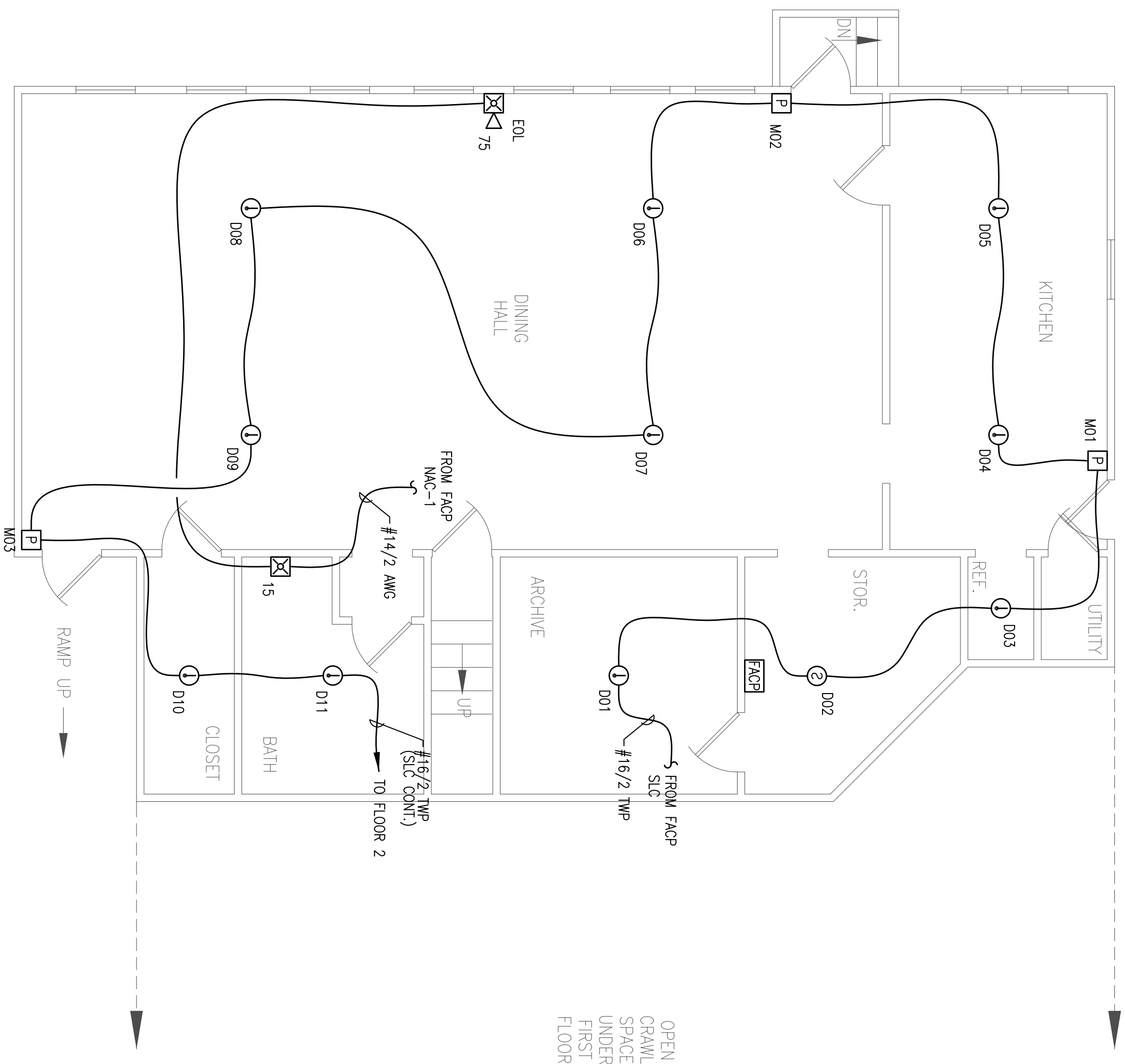
PLAN NORTH FLOOR "B" FIRE ALARM PLAN SCALE: 1/4"=1'-0" FIELD VERIFY DIMENSIONS
