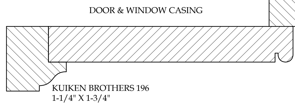
5 NEW CASING AT WINDOWS & DOORS A-1.8 Scale: FULL SIZE
