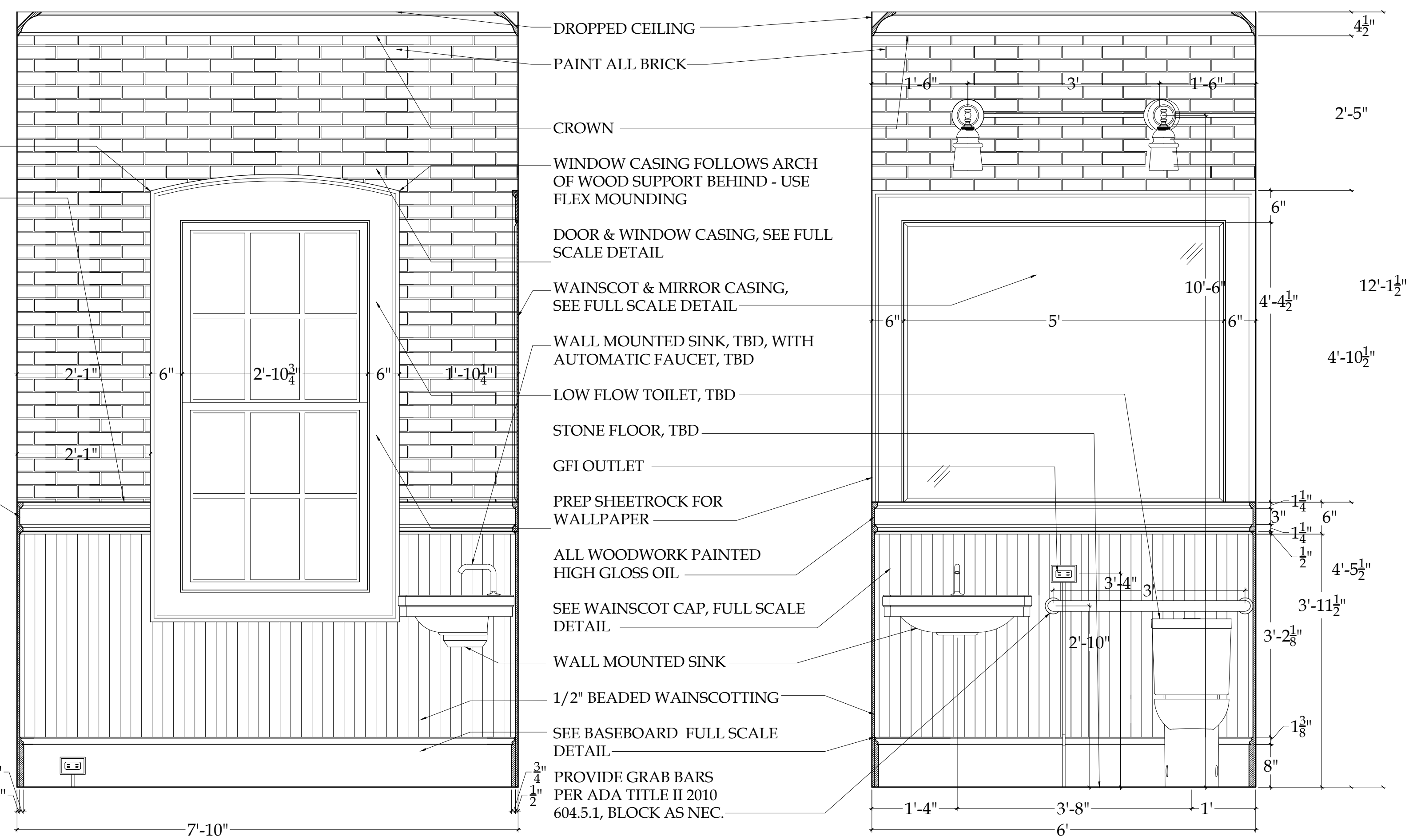
3 RESTROOM: EAST ELEV. Scale: 3/4"=1'-0"
