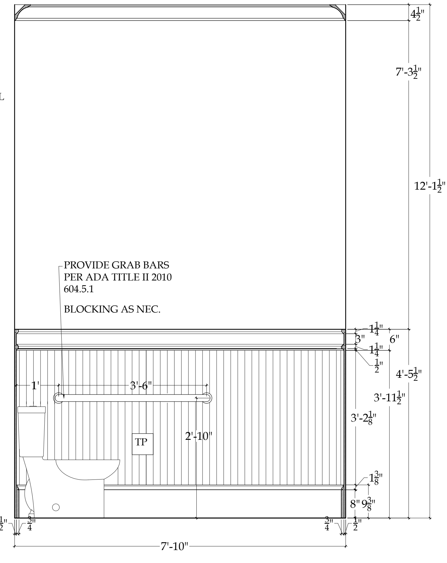
6 RESTROOM: WEST ELEV. Scale: 3/4"=1'-0"
