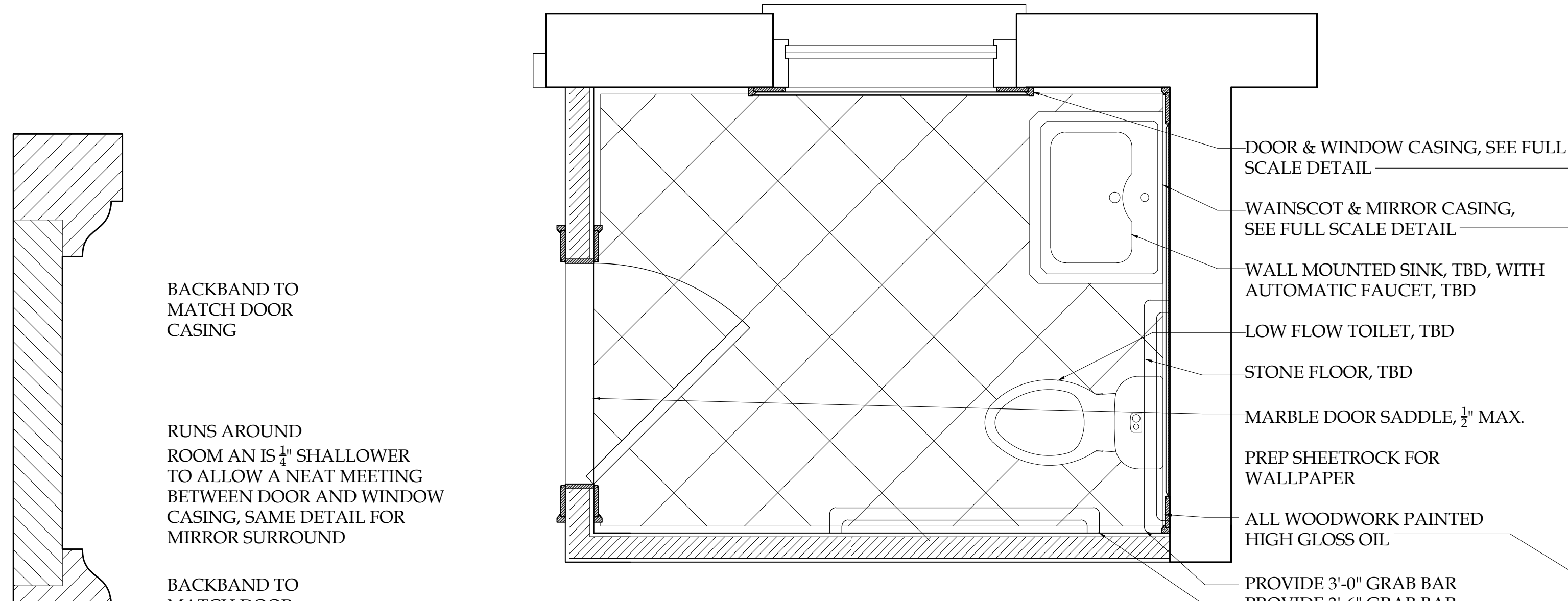
1 RESTROOM: PLAN SECTION Scale: 3/4"=1'-0"
