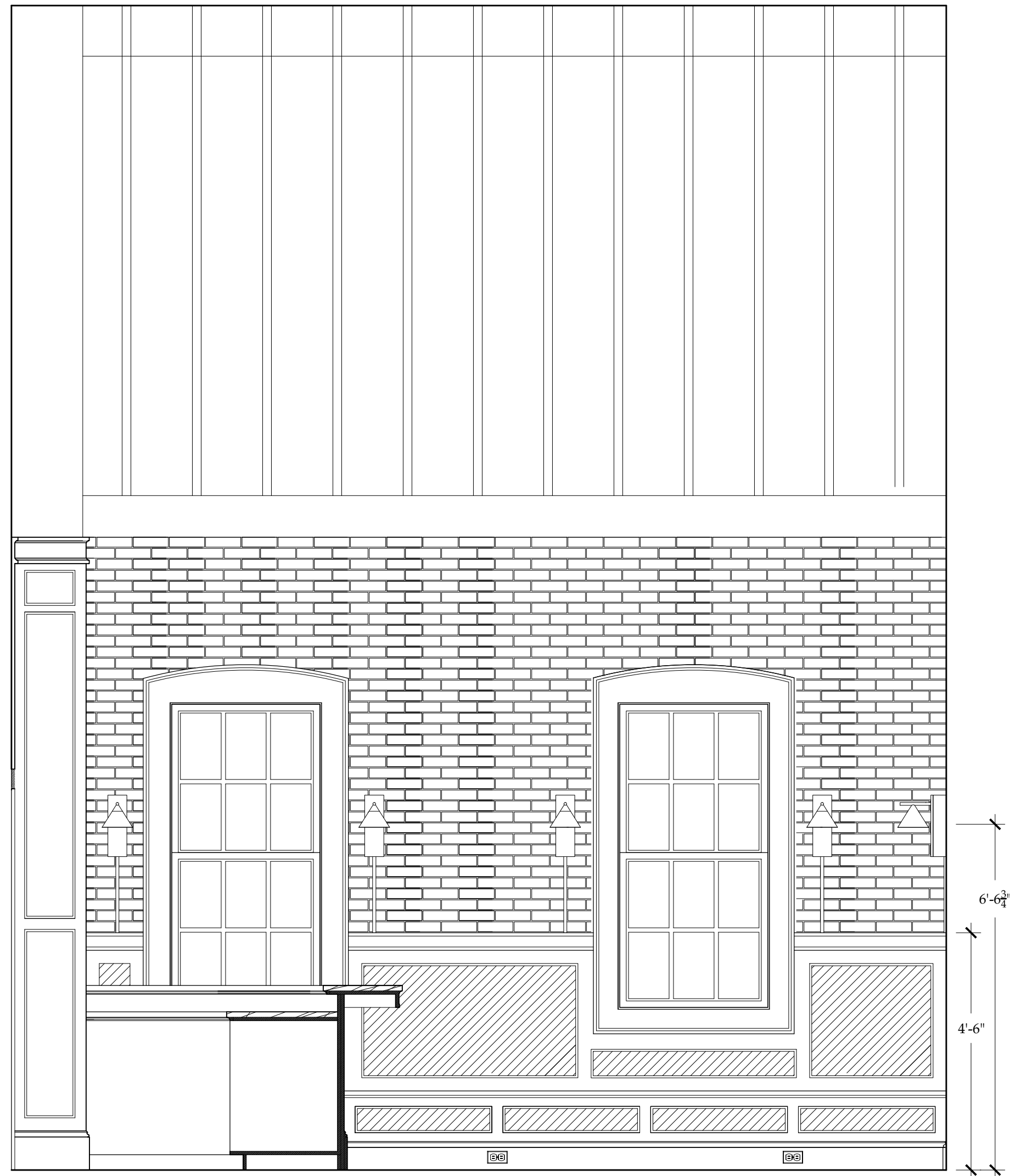
1 MAIN DINING ROOM: EAST ELEVATION 1-1.1 Scale: 1/2"=1'-0"
