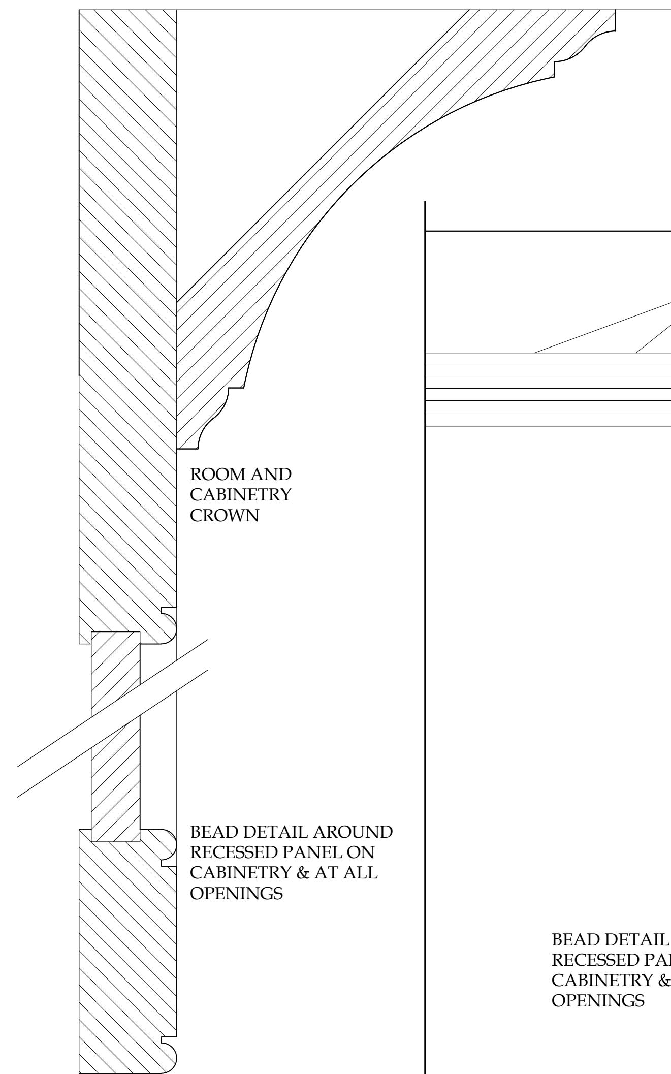
1 UPPER CABINET DETAIL A-1.8 Scale: FULL SIZE
