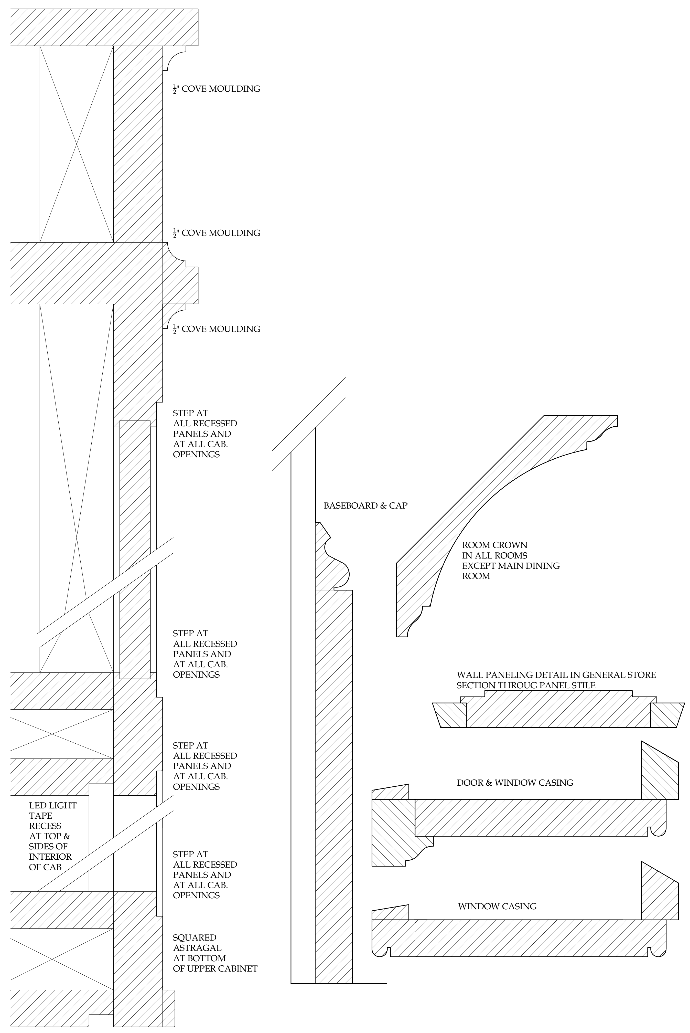
1 CABINETS: DETAIL FOR CABINETS AT BARS I-1.8B Scale: FULL SIZE
