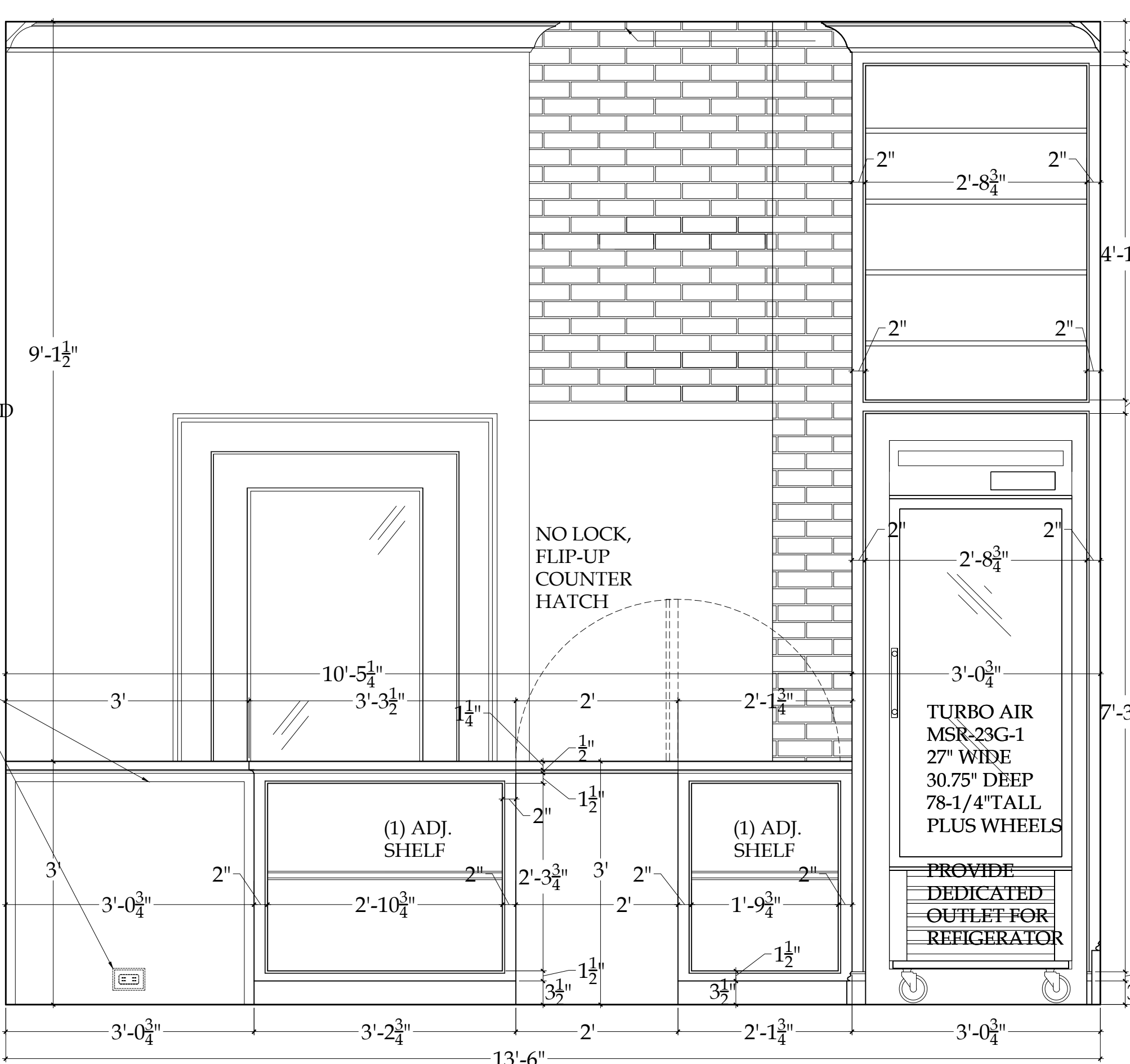
7 1-1.6 GENERAL STORE: SOUTH ELEV. FRONT COUNTER (SERVICE SIDE) Scale: 3/4"=1'-0"
