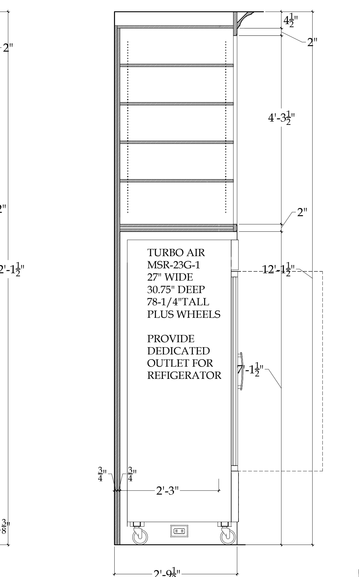
8 1-1.6 GENERAL STORE: SECTION THRU TALL STORAGE CABINET Scale: 3/4"=1'-0"
