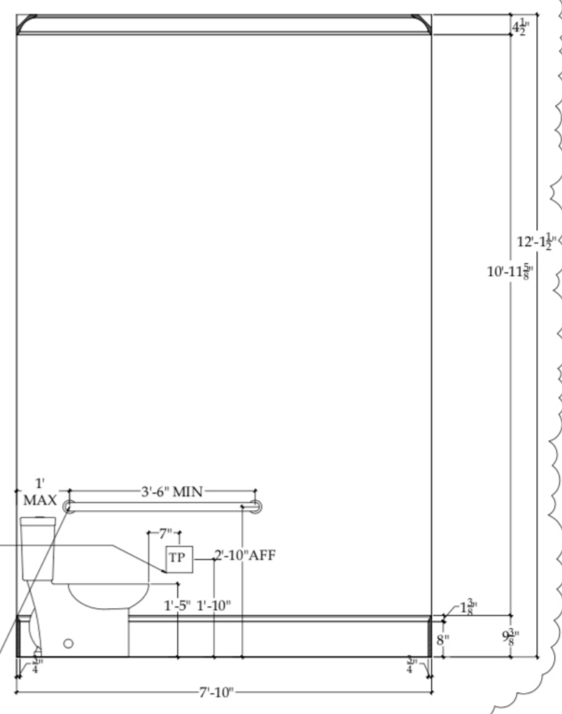
6 1-1.5 RESTROOM: WEST ELEV. Scale: 3/4"=1'-0"
