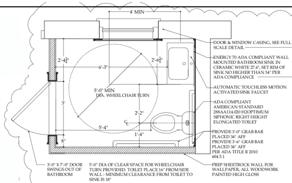
1 1-1.5 RESTROOM: PLAN SECTION Scale: 3/4"=1'-0"
