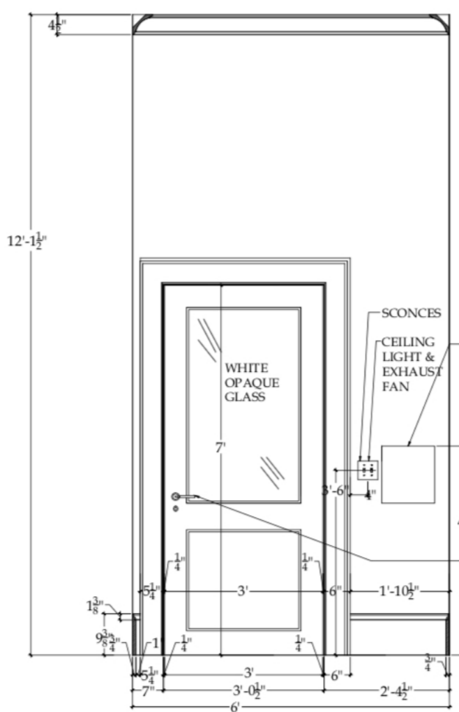
5 1-1.5 RESTROOM: NORTH ELEV. Scale: 3/4"=1'-0"
