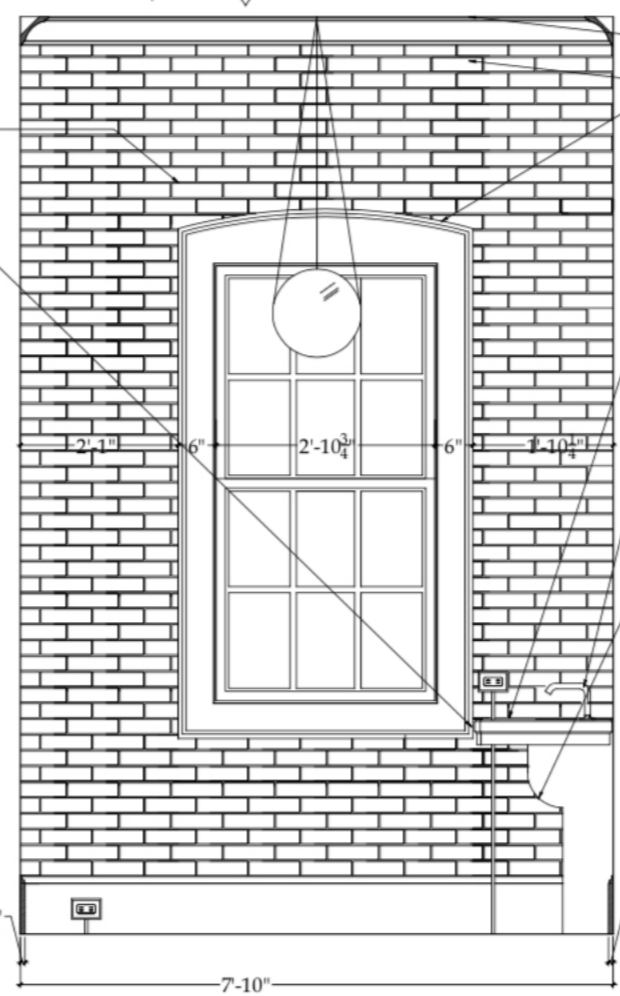
3 1-1.5 RESTROOM: EAST ELEV. Scale: 3/4"=1'-0"
