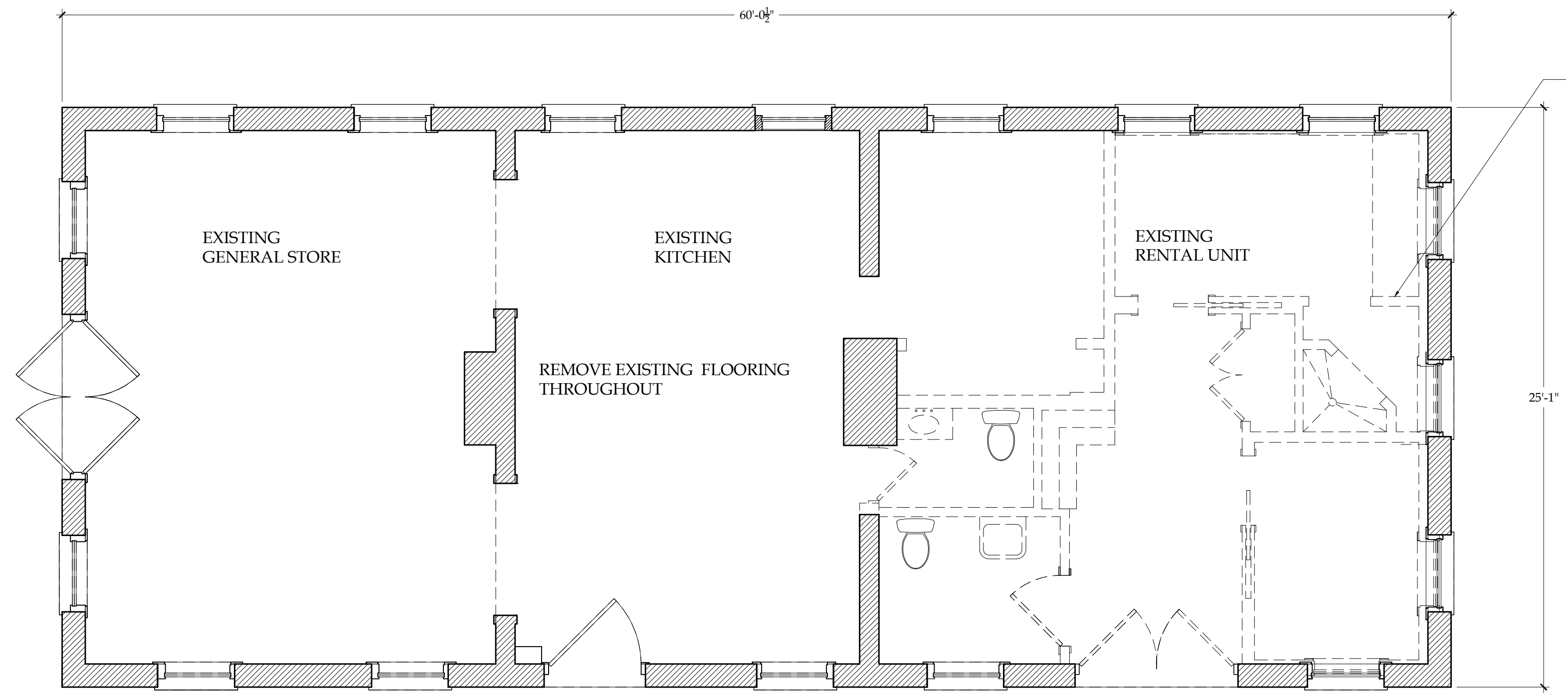
1 DEMO PLAN VIEW DEMO Scale: 1/4"=1'-0"
