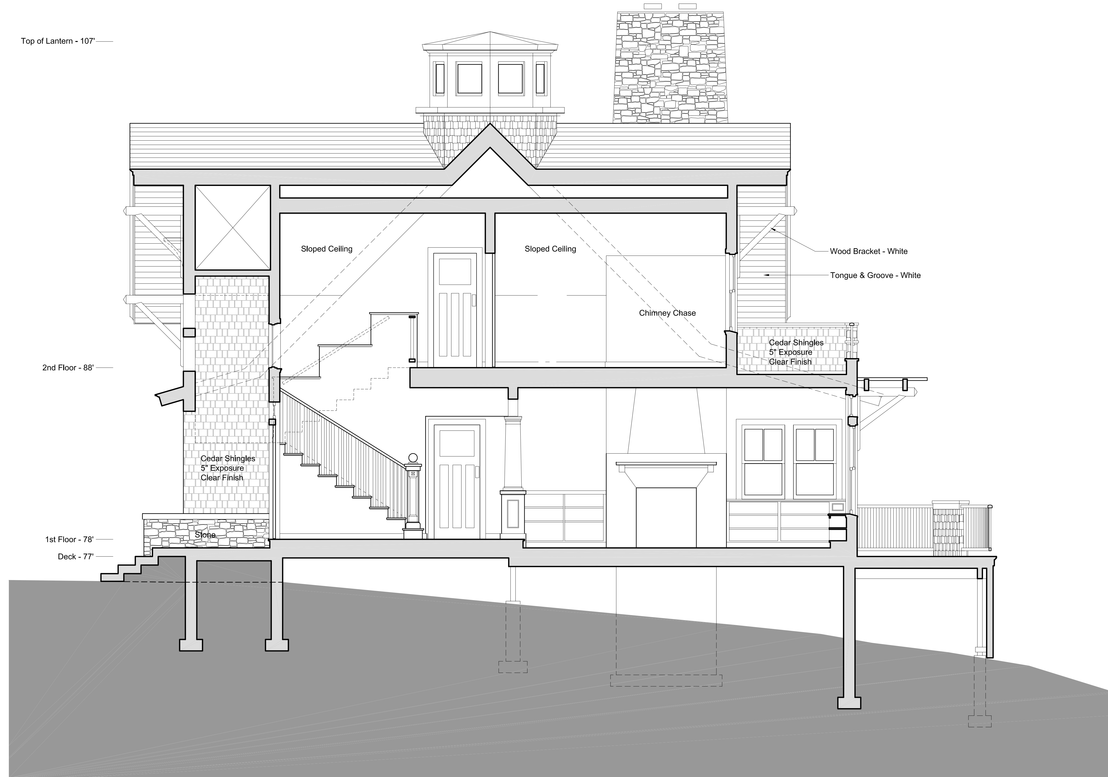
1 SECTION B - THROUGH ENTRY HALL & LIVING ROOM 1/4" = 1'-0"
