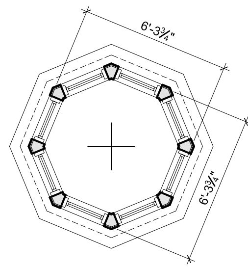
1 SKYLIGHT 1/4" = 1'-0"
