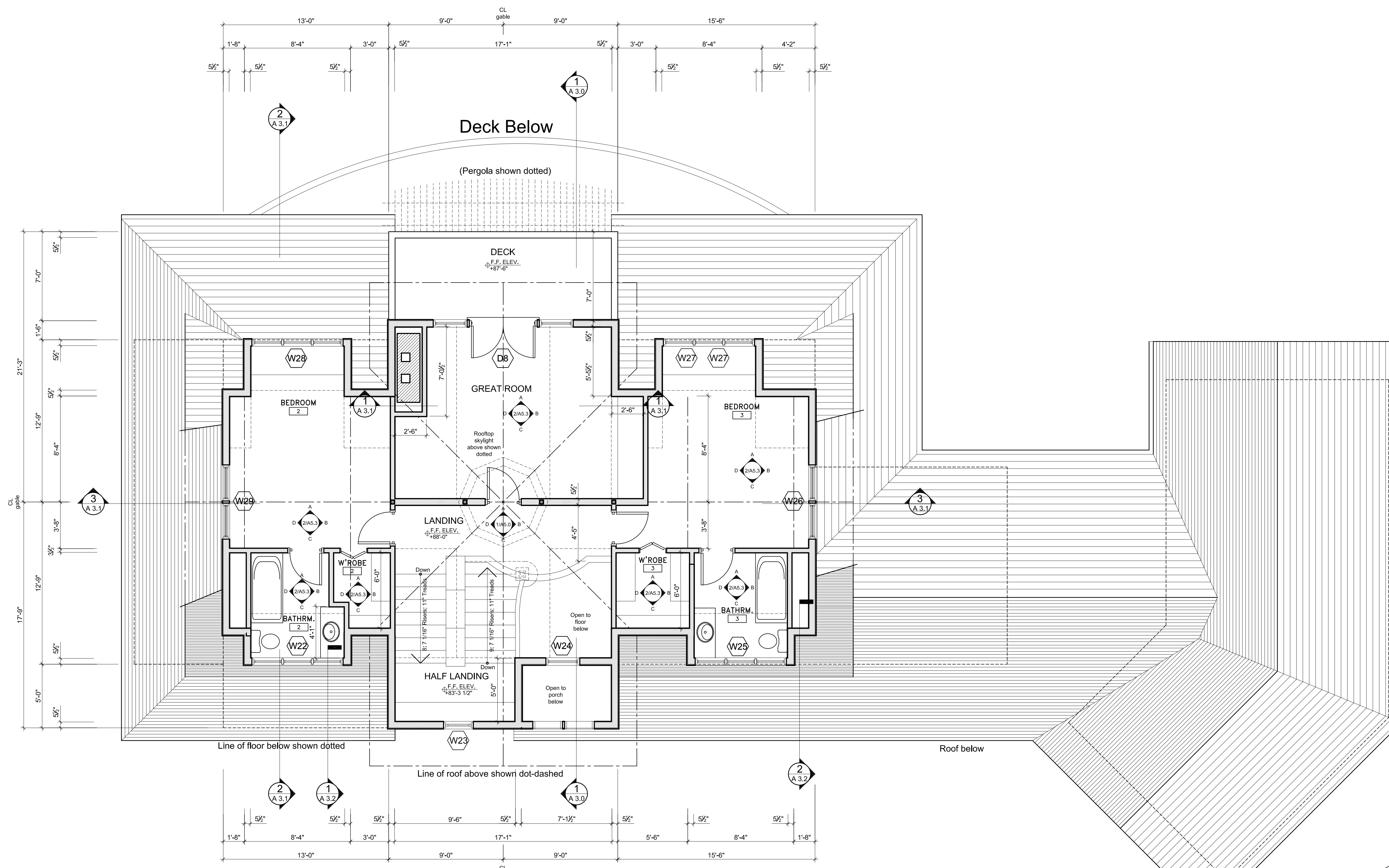
2 2ND. FLOOR LAYOUT 1/4" = 1'-0"
