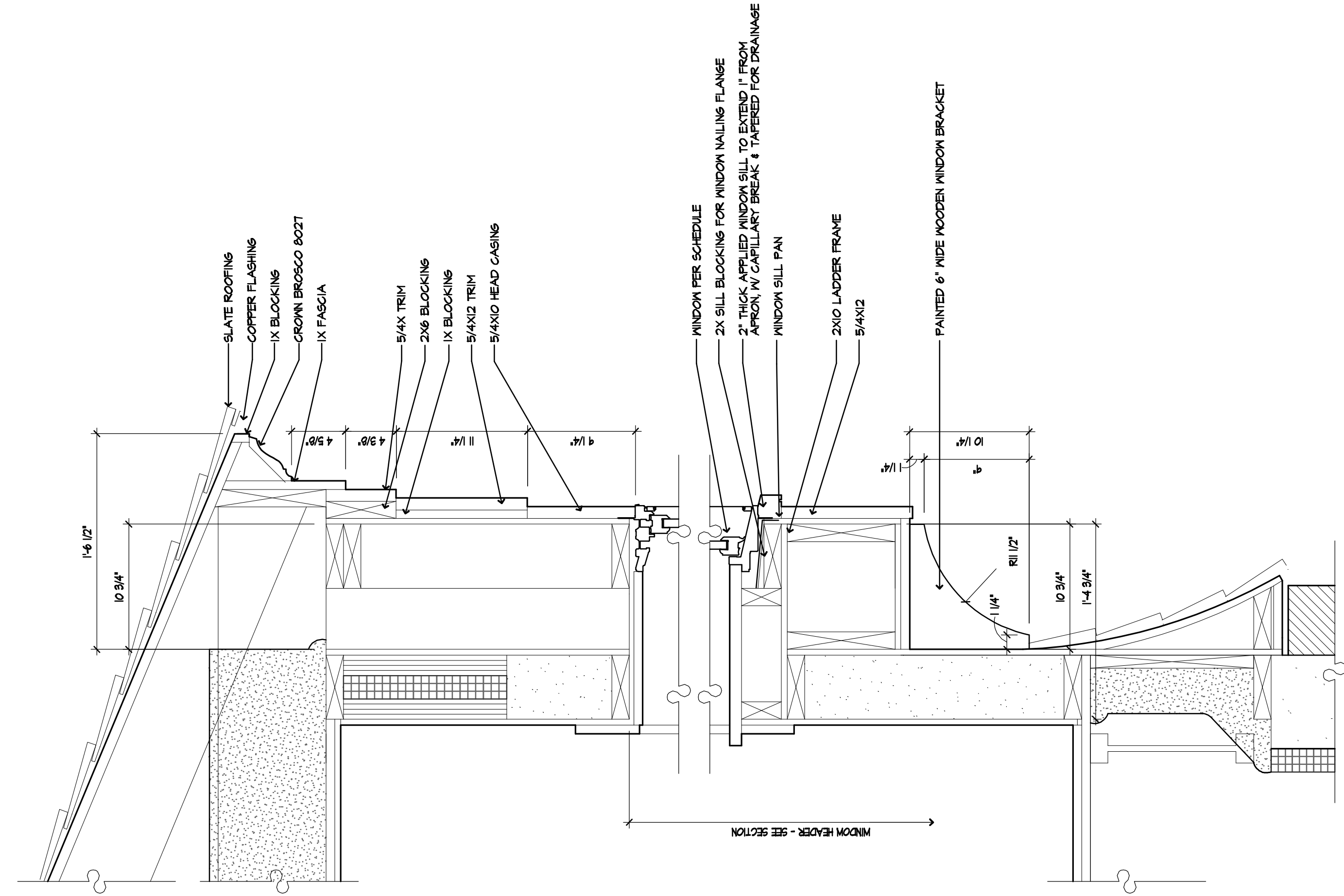
2 BOXED WINDOW DETAIL A4.1 1/12" = 1'-0"
