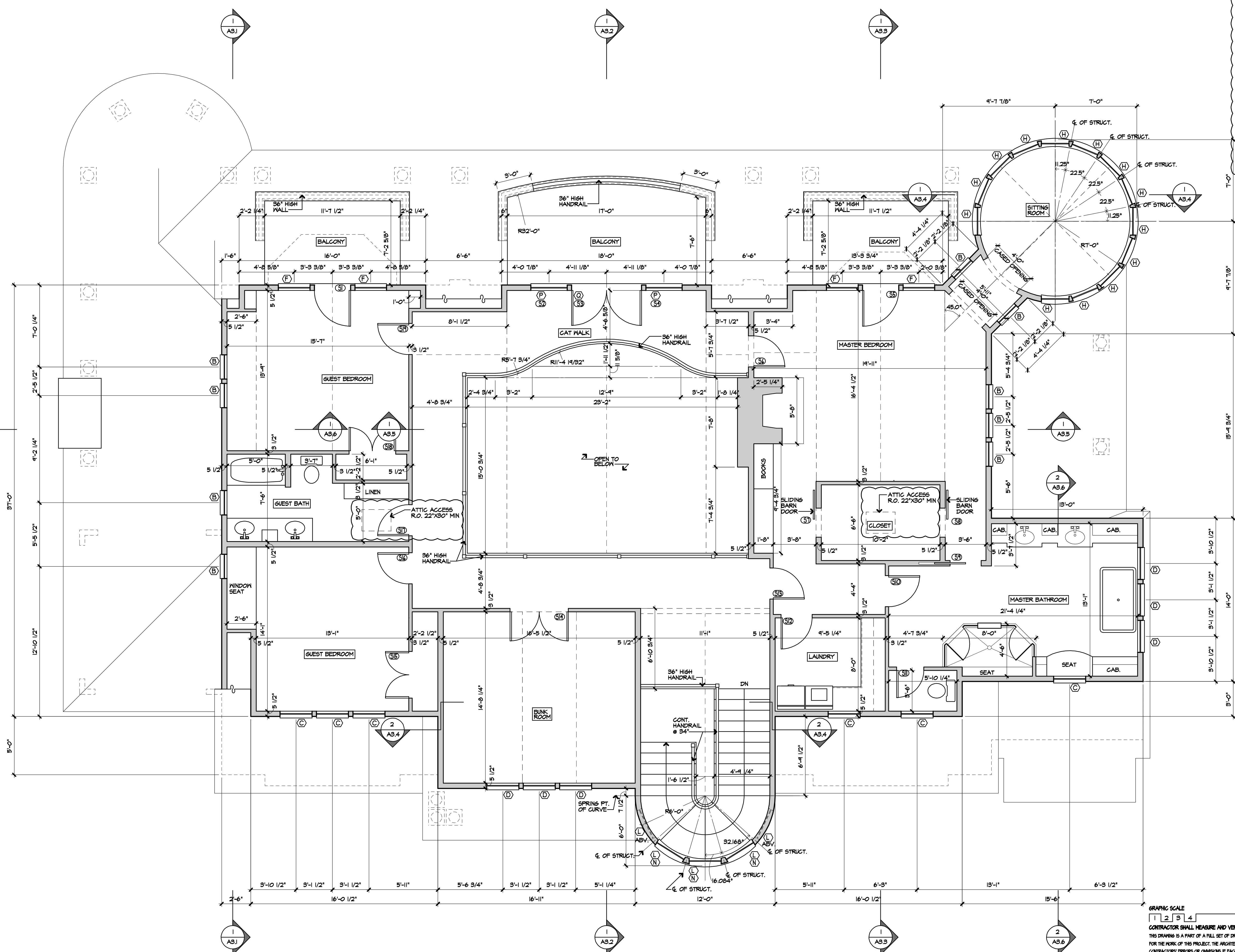
1 SECOND FLOOR PLAN A1.3 1/4" = 1'-0"
