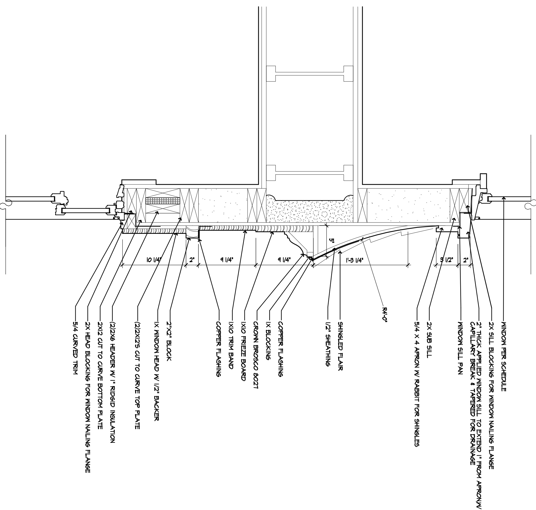
2 TYPICAL WINDOW FRAMING PLAN @ TURRET A4.3 1/12" = 1'-0"
