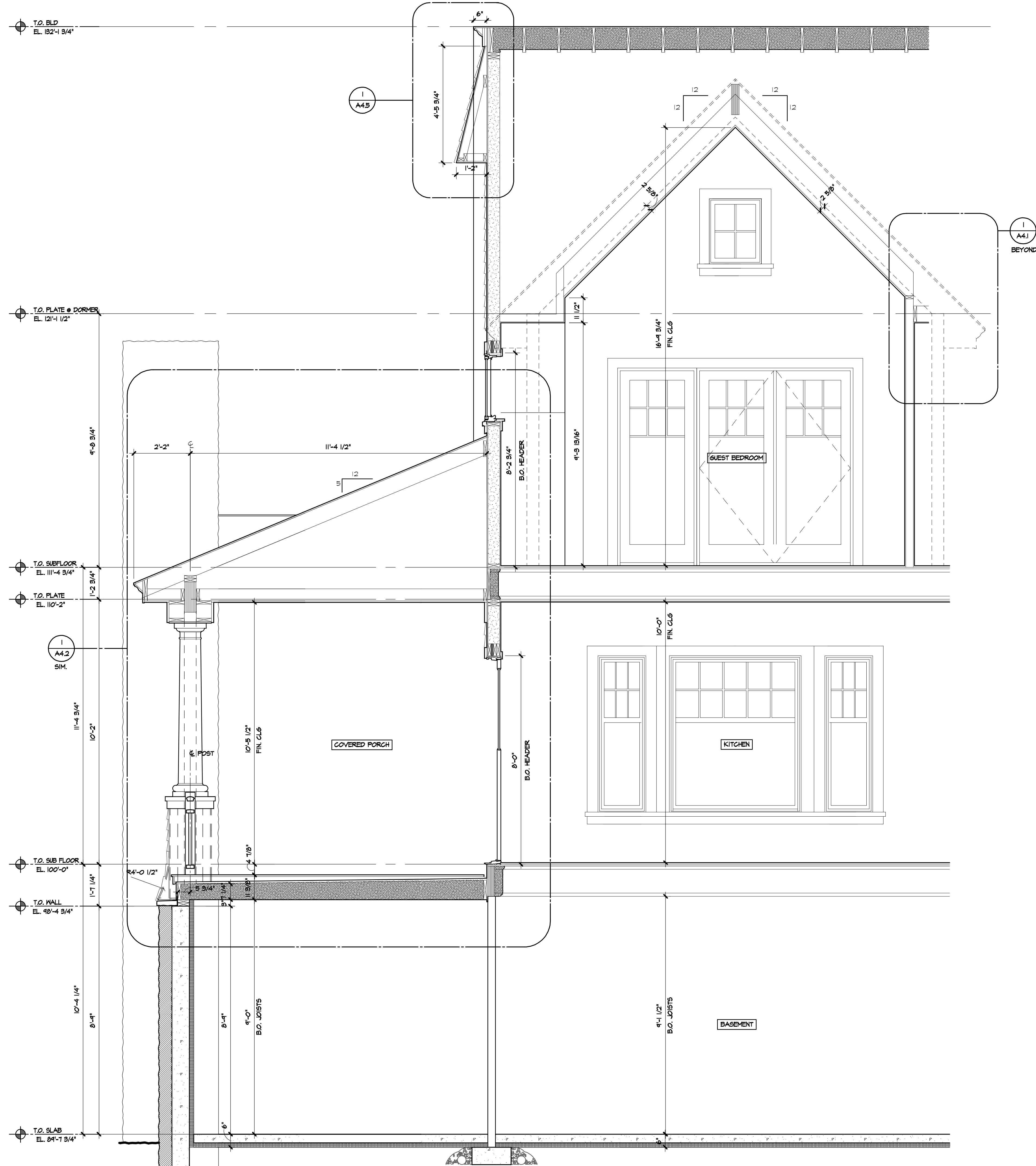
1 CROSS-SECTION A3.6 1/2" = 1'-0"
