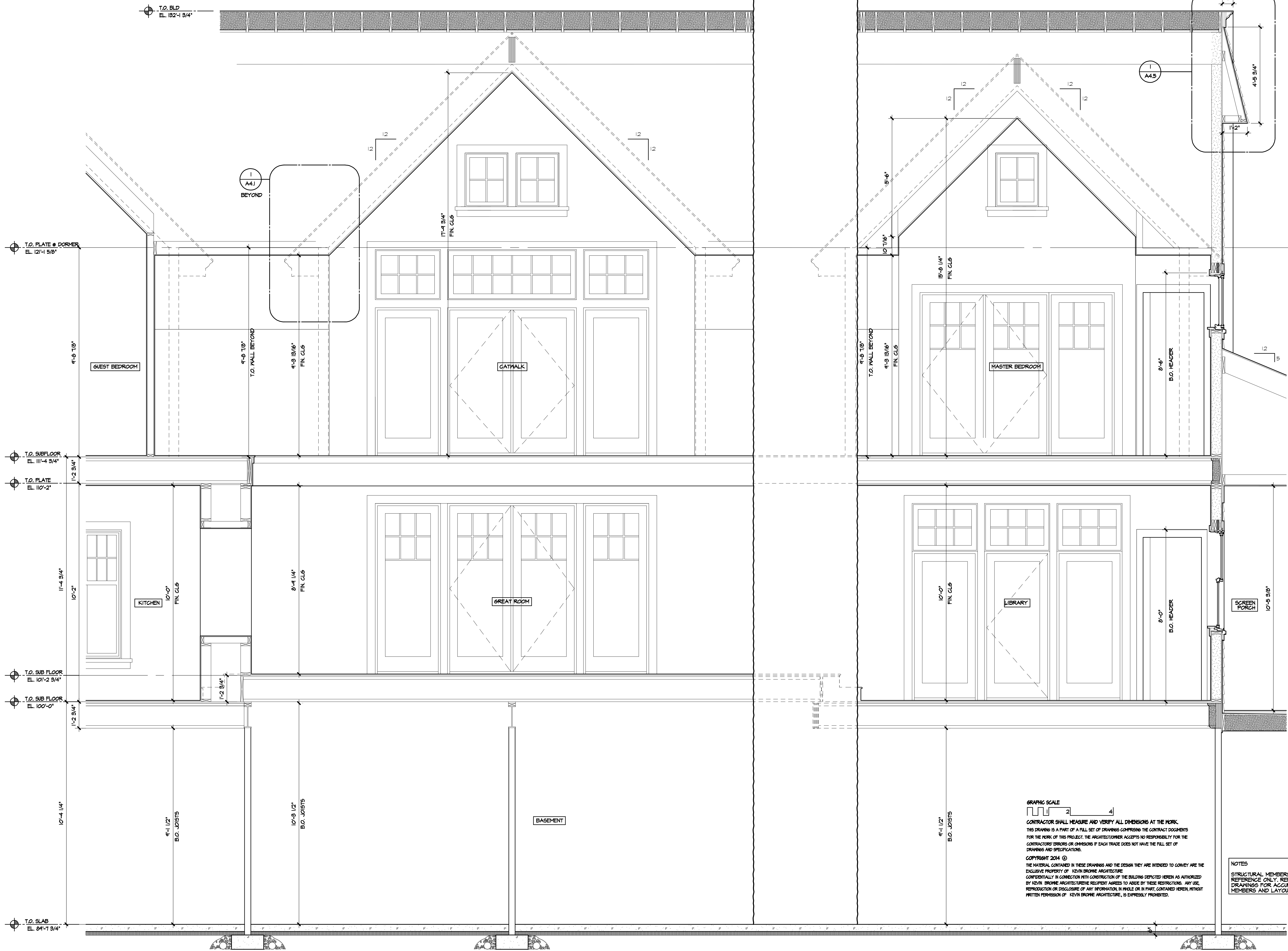
1 CROSS-SECTION A3.5 1/2" = 1'-0"
