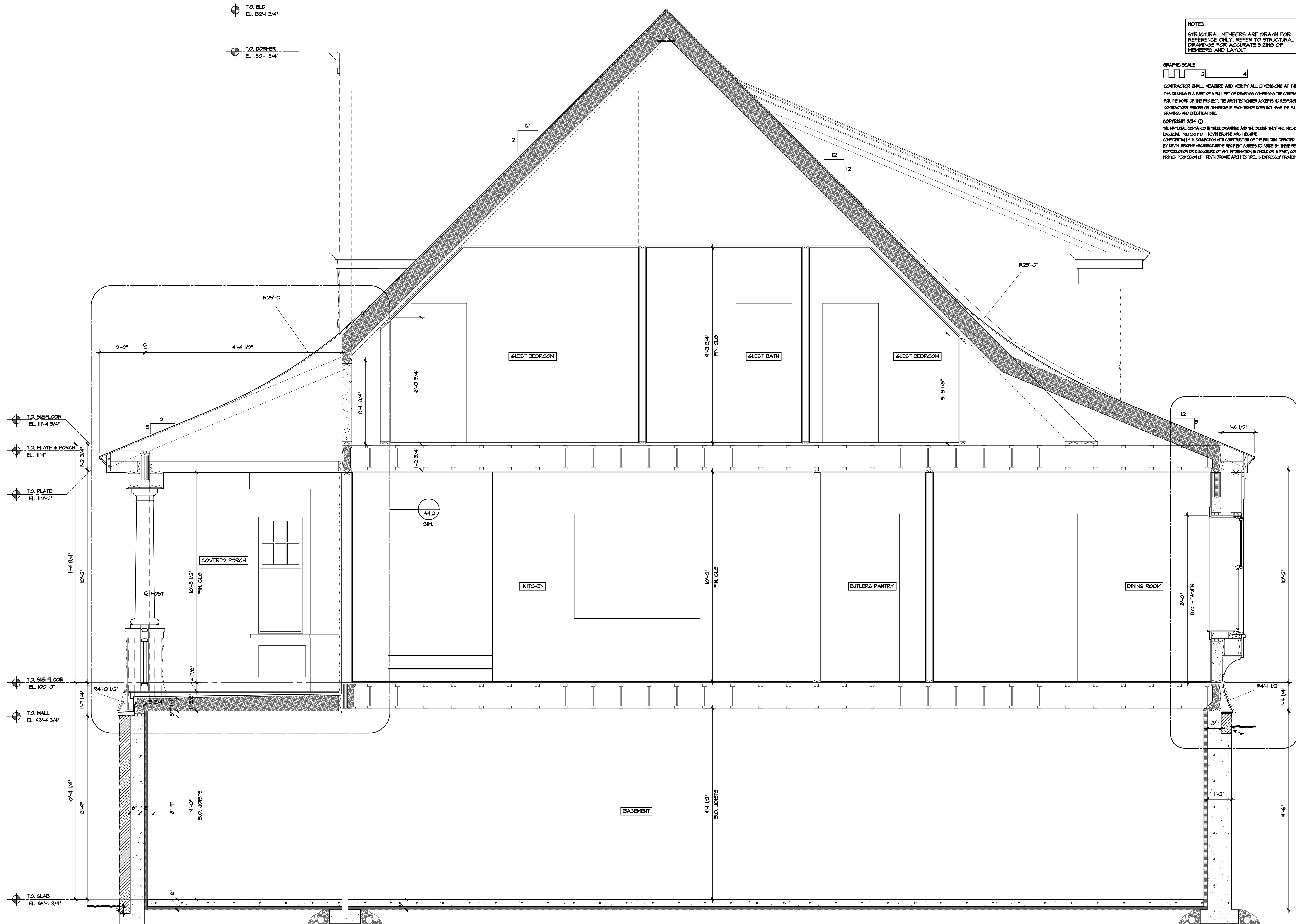
1 CROSS-SECTION A3.1 1/2" = 1'-0"
