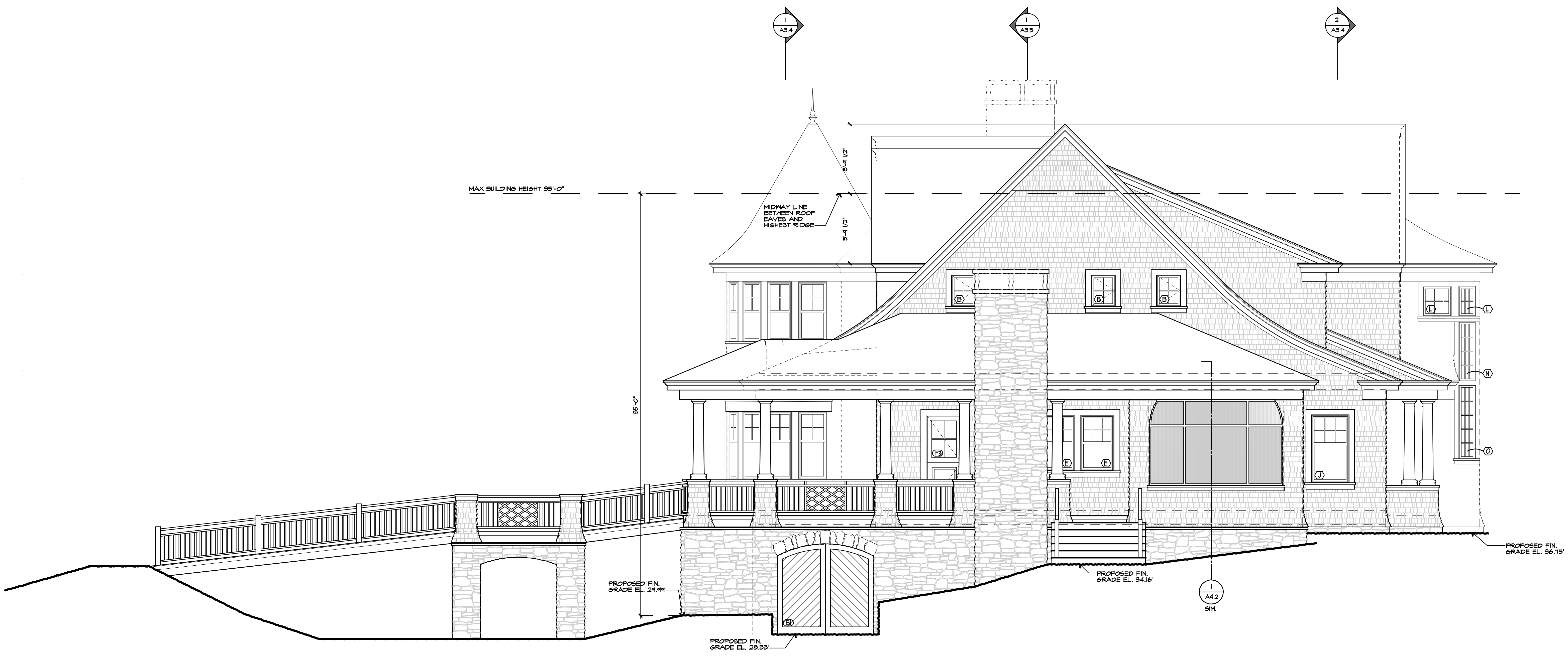
1 ELEVATIONS A2.4 1/4" = 1'-0"
