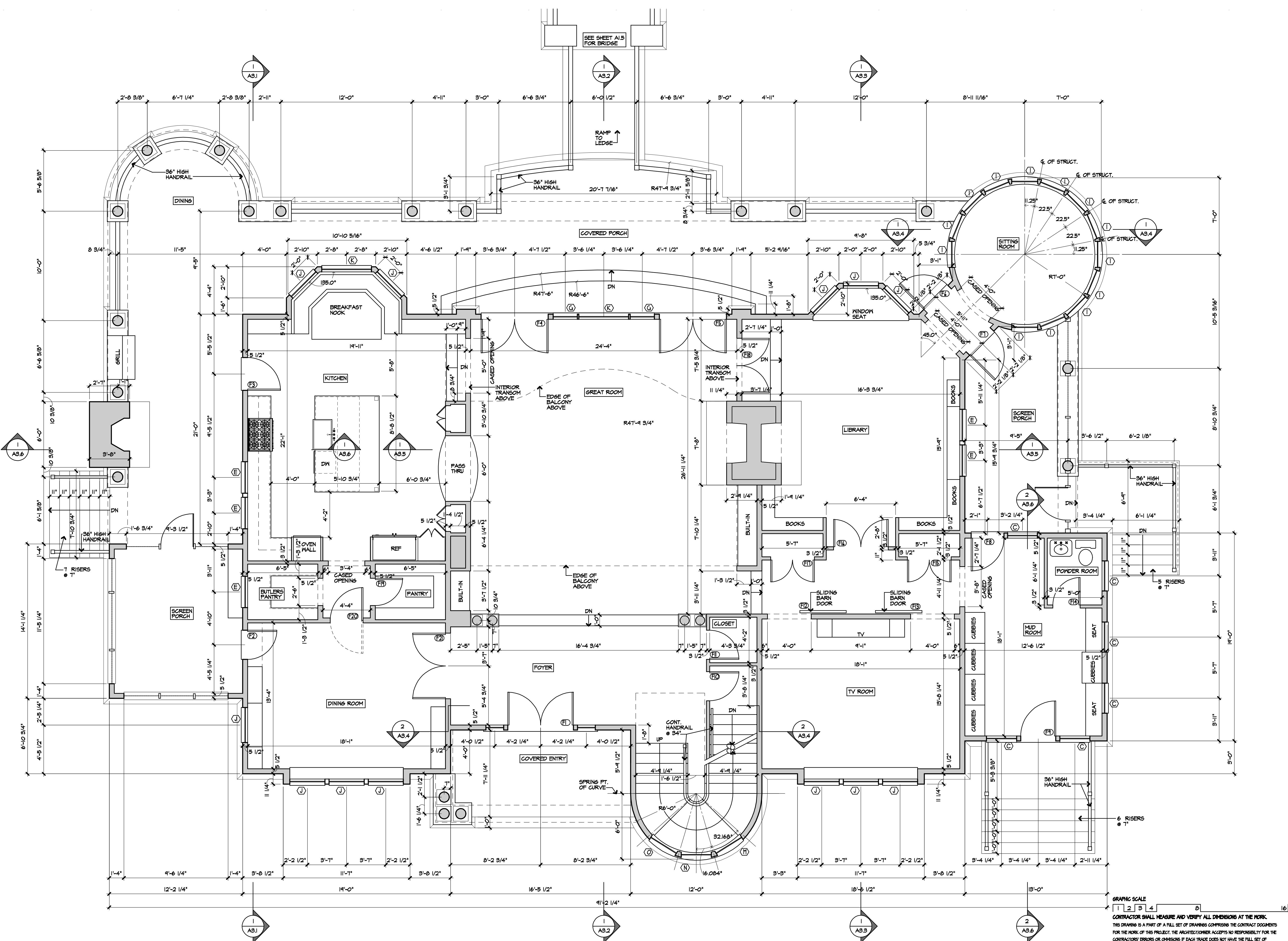
1 FIRST FLOOR PLAN A1.2 1/4" = 1'-0"
