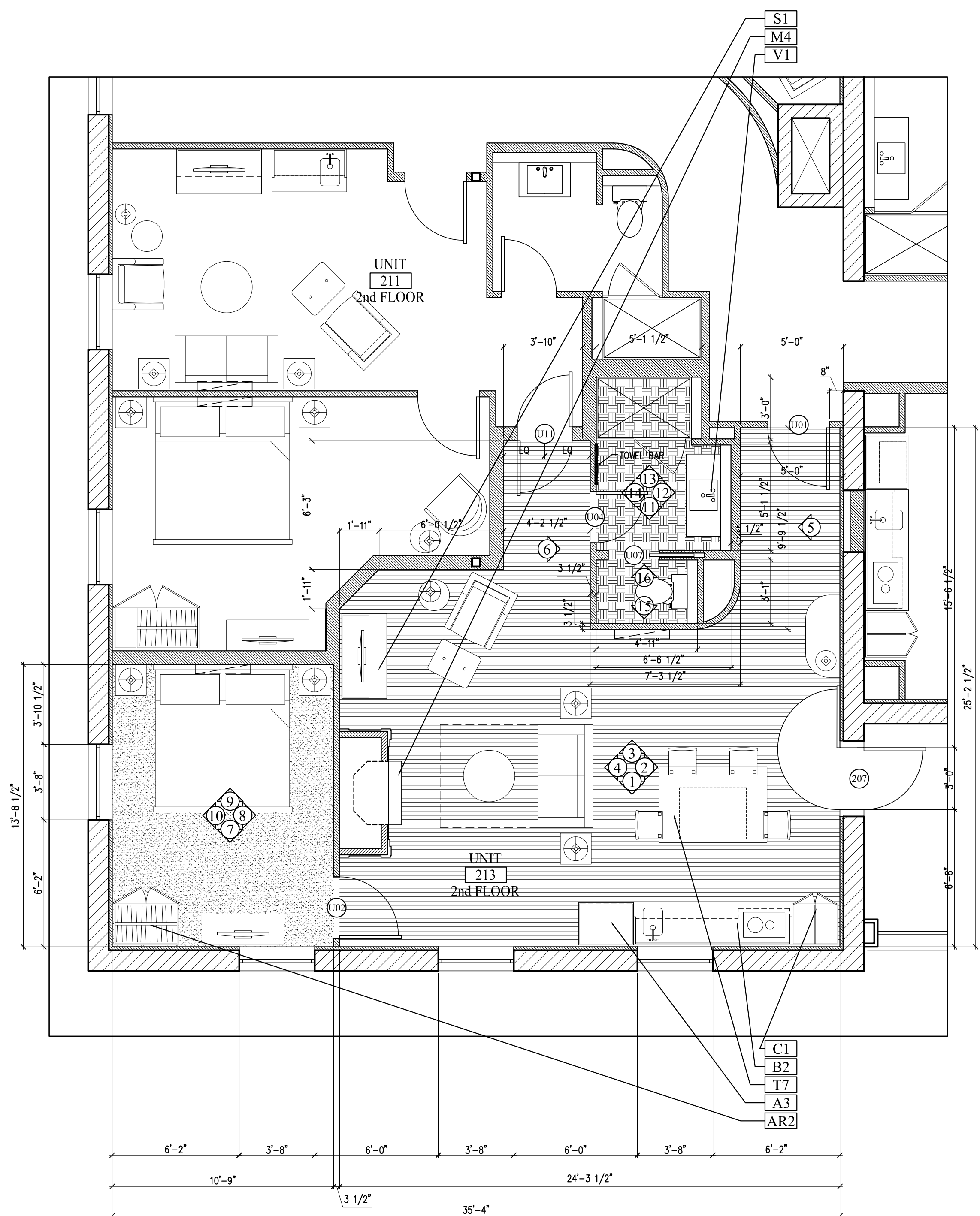
A ENLARGED FLOOR PLAN UNIT 213 SECOND FLOOR 1/4"=1'-0"
