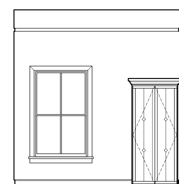
7 INTERIOR ELEVATION UNIT 213 1/4"=1'-0"
