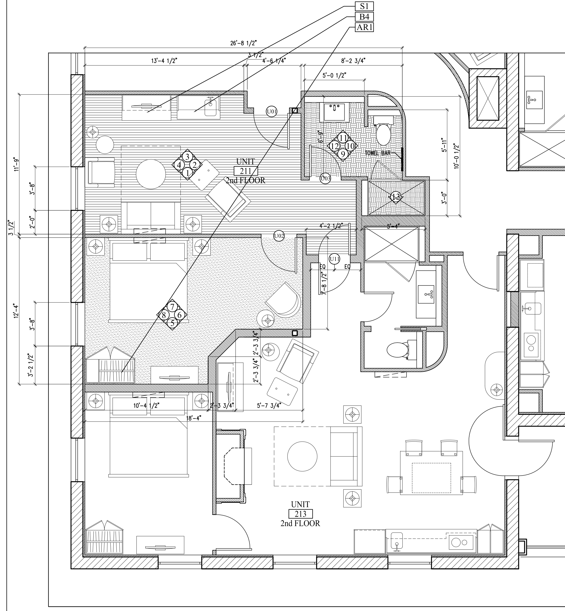
A ENLARGED FLOOR PLAN UNIT 211 SECOND FLOOR 1/4"=1'-0"
