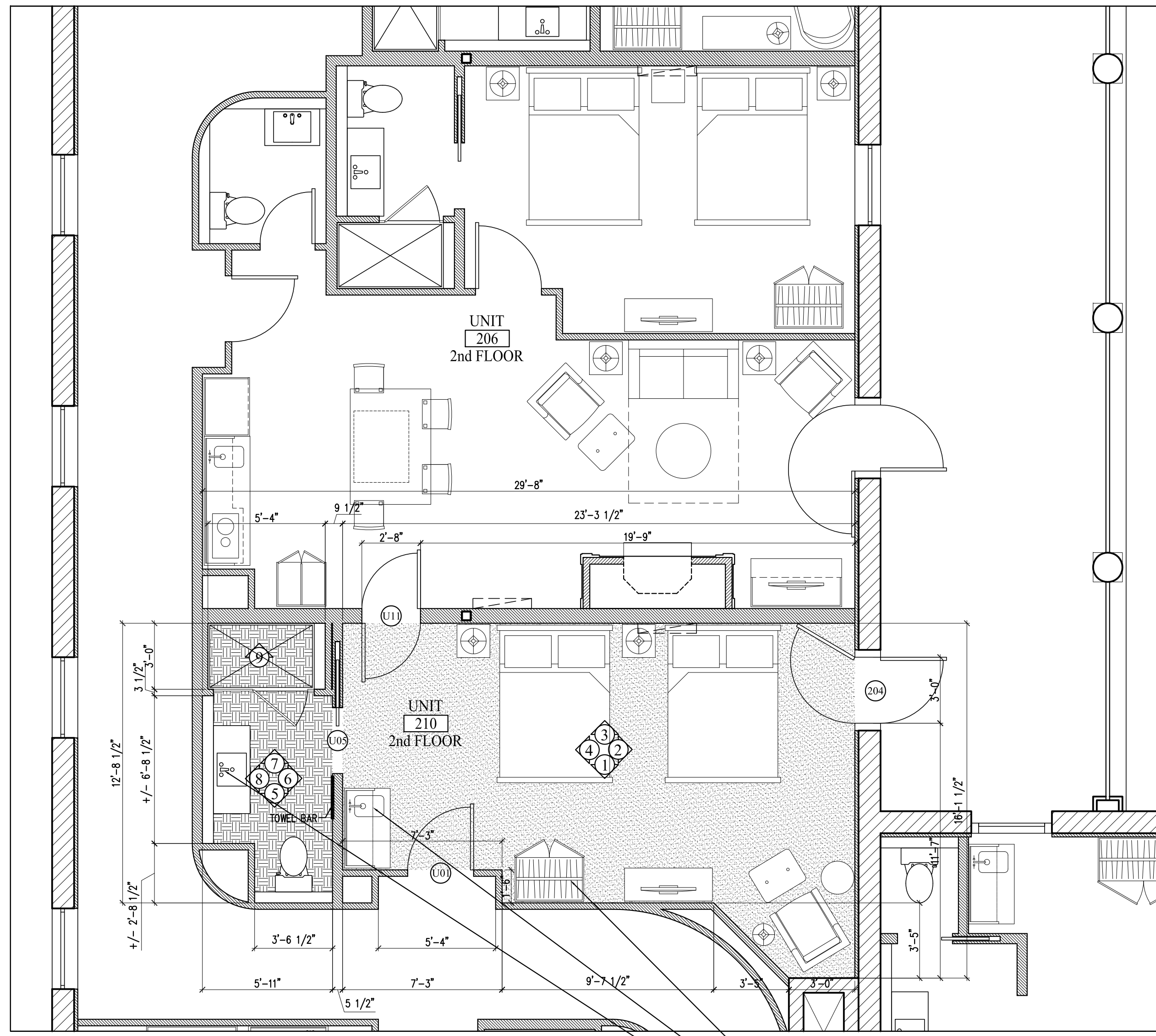
A | ENLARGED FLOOR PLAN UNIT 210 SECOND FLOOR 1/4"=1'-0"
