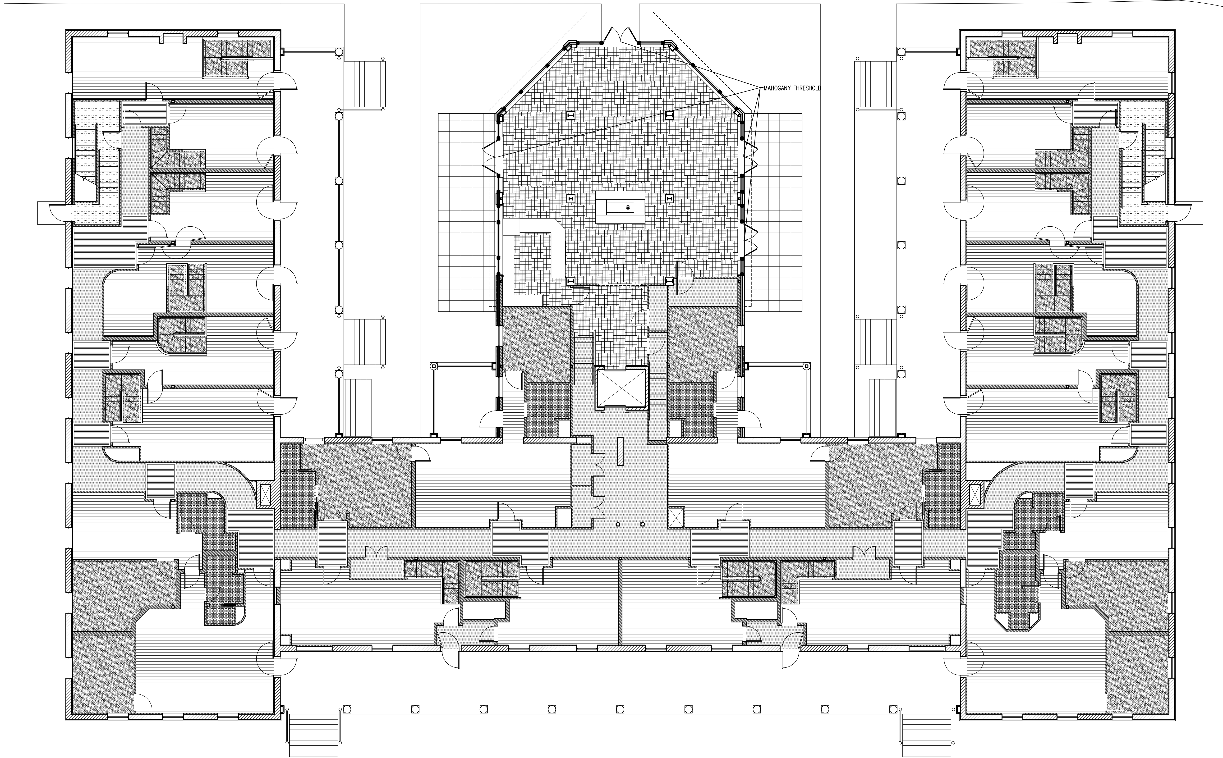
1 | FIRST FLOOR FLOOR FINISH SCHEDULE SCALE: 1/8"=1'-0"
