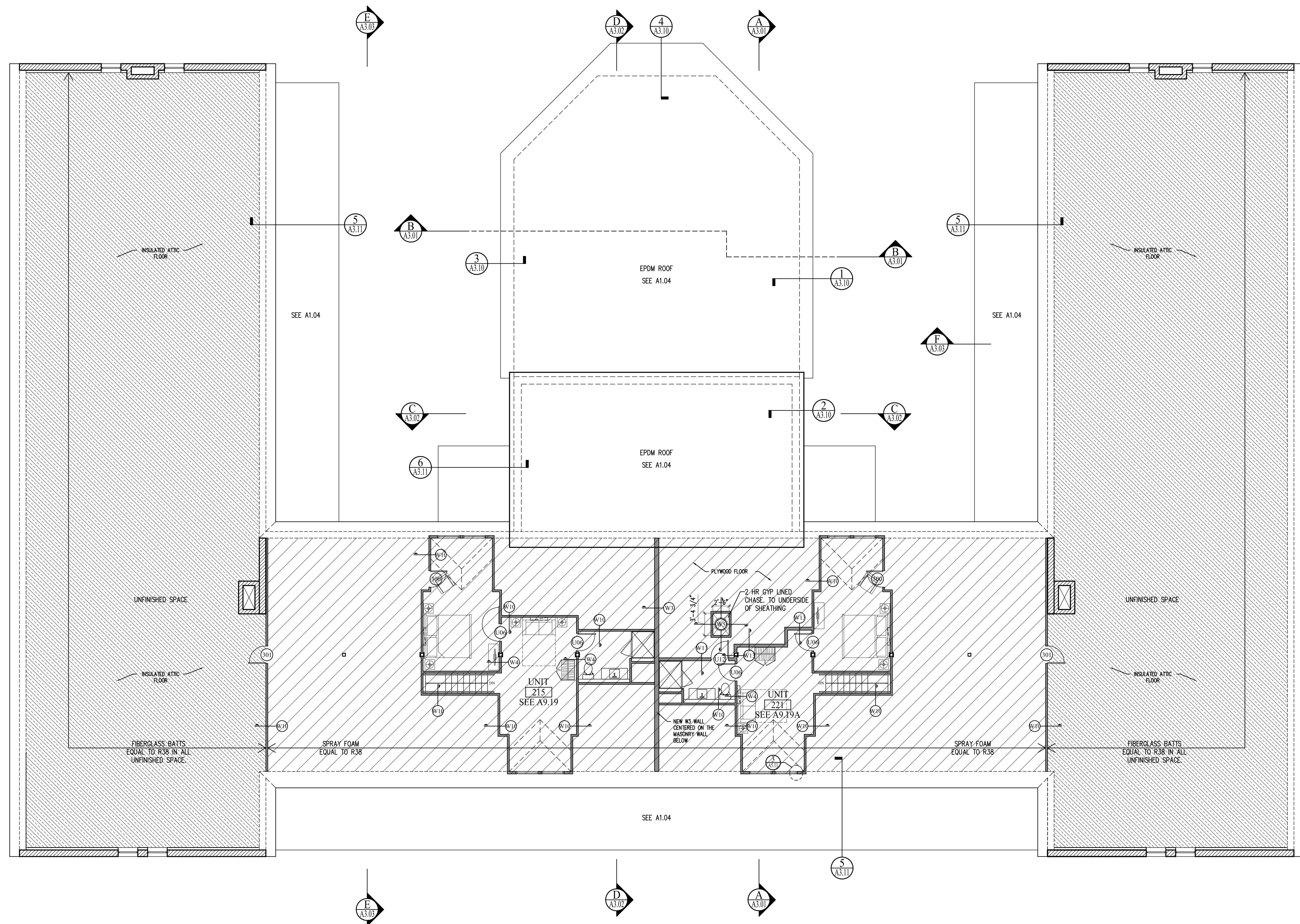
1 | THIRD FLOOR PLAN / ATTIC PLAN SCALE: 1/8"=1'-0"
