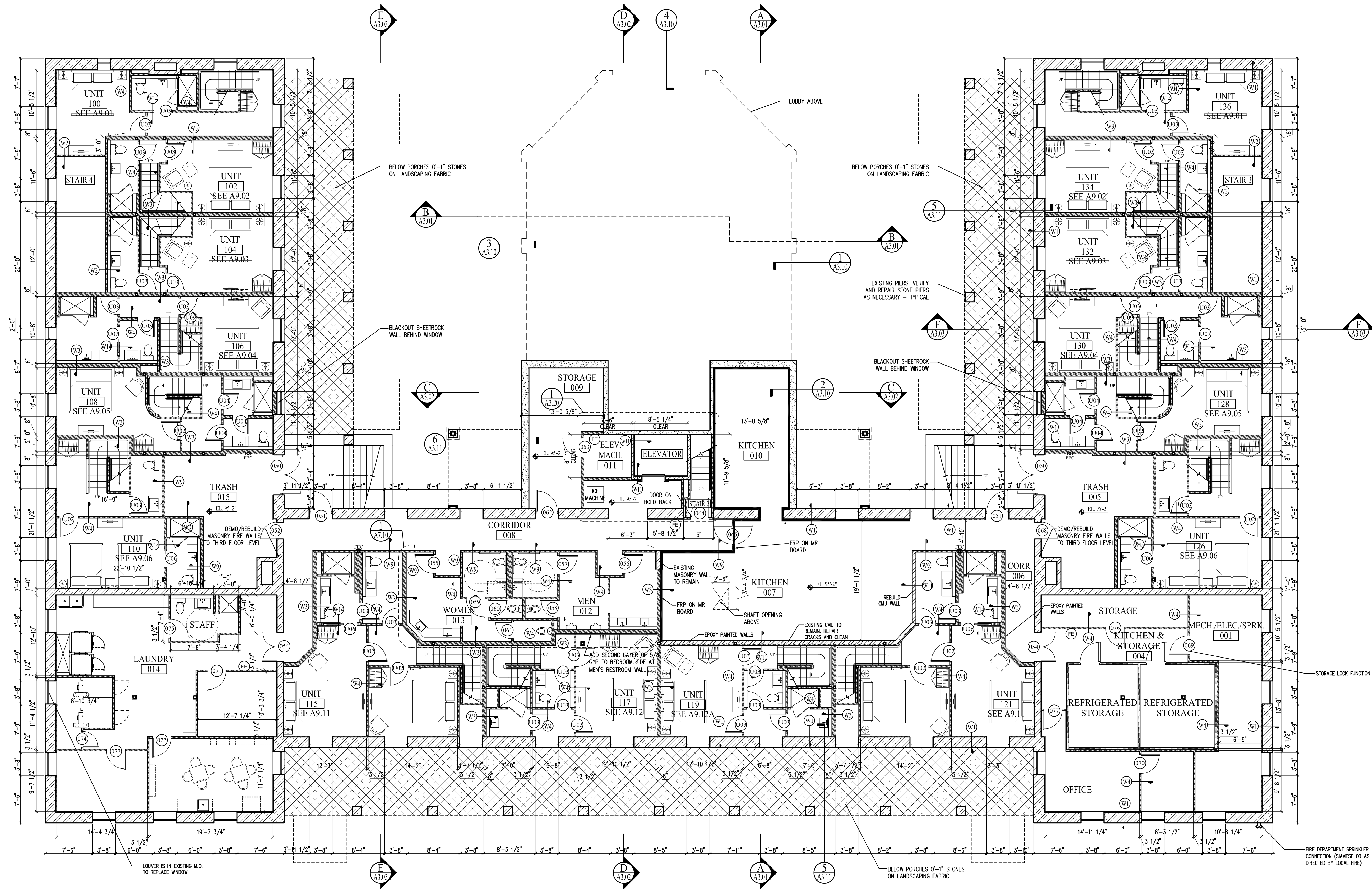
1 BASEMENT PLAN SCALE: 1/8"=1'-0"
