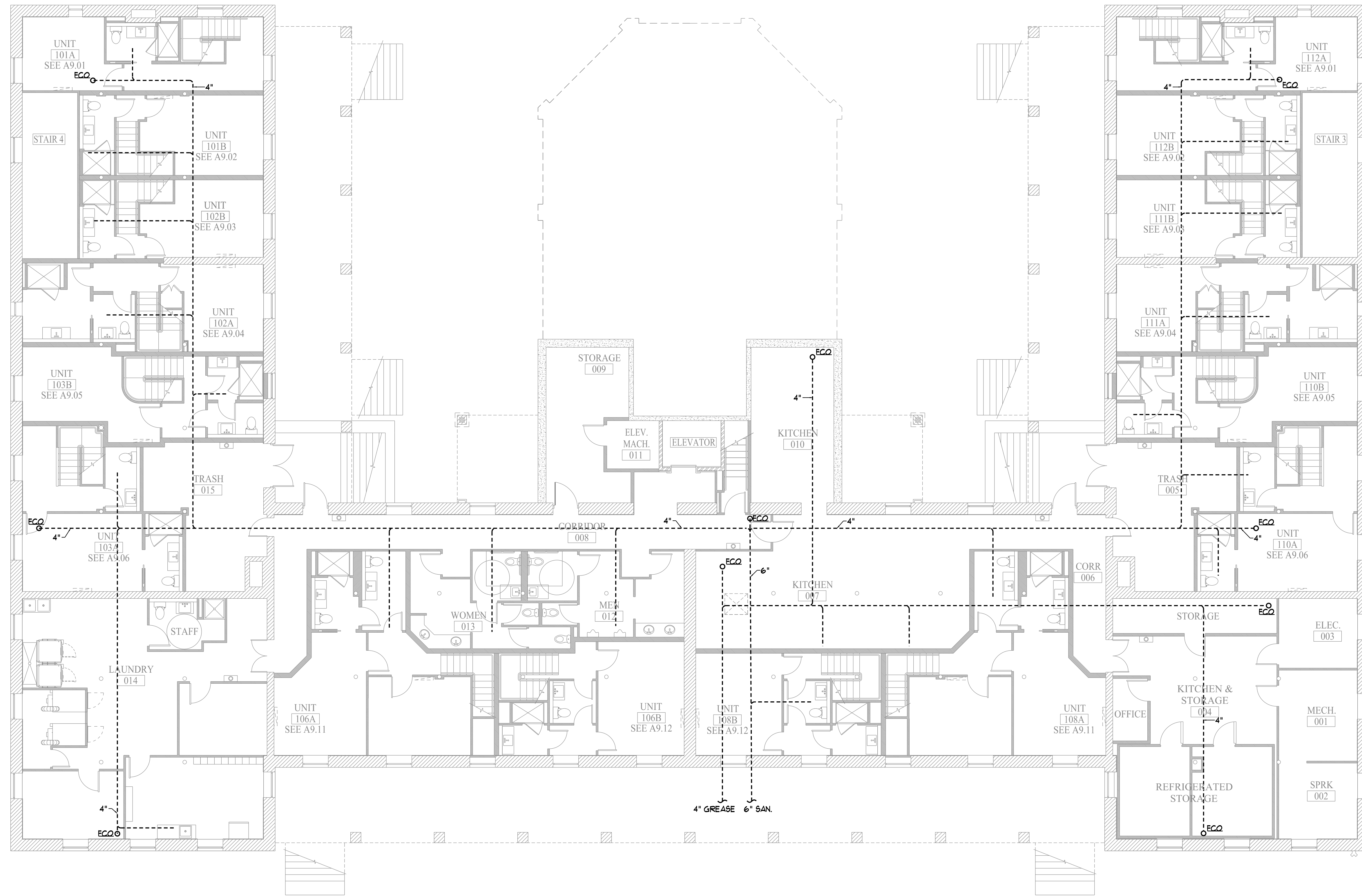
BASEMENT PLUMBING PLAN SCALE 1/8" = 1'-0"
